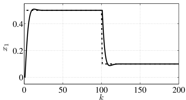
Figure 4.11: Tracking of the reference \bar{x}_1(k) . Solid line: tracking response of x_1(k) . Dash-dotted line: reference.
