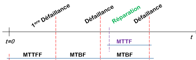
FIGURE 1.13 – MTTFF, MTBF, MTTF
