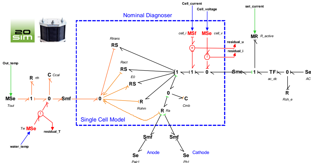
Figure 3.14 – Electrolyser BGD
