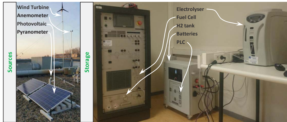
Figure 4.2 – Experimental HRES for hydrogen production and storage
