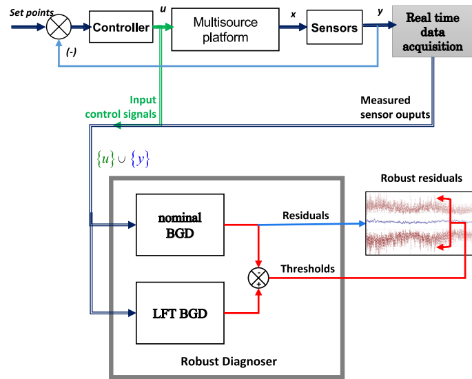
Figure 3.17 – Nominal and LFT BGD coupling
