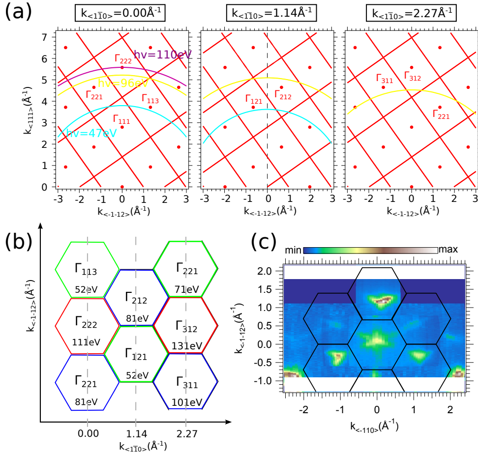
Figure 5.5: (a) Bulk reciprocal lattice of SrTiO 3 in the k_{(111)} - k_{(112)} plane for different k_{(110)} values as indicated in (b). Practically, different k_{(110)} values are chosen by rotating the sample. The pink, yellow and cyan lines correspond to the cuts in reciprocal space measured by ARPES at the specified photon energies. If the cut is close to a \Gamma point, the states corresponding to the 2DES have non-zero ARPES intensities. (b) Reciprocal 2D space in the (111) plane. Inside each Brillouin zone the projections of the different bulk \Gamma points corresponding to available final states during the photoemission process at the specified photon energy are indicated. The color (red, blue, green) of the hexagons indicates which \Gamma points are located in the same (111) plane in reciprocal space. The figures in (a,b) help understanding the Fermi-surface intensities shown in panel (c). (c) Superposition of Fermi surface maps measured for in situ prepared SrTiO 3 (111) sample ( (3 \times 3) reconstructed surface) at photon energies of h\nu = 47 \text{ eV} and h\nu = 96 \text{ eV} .
