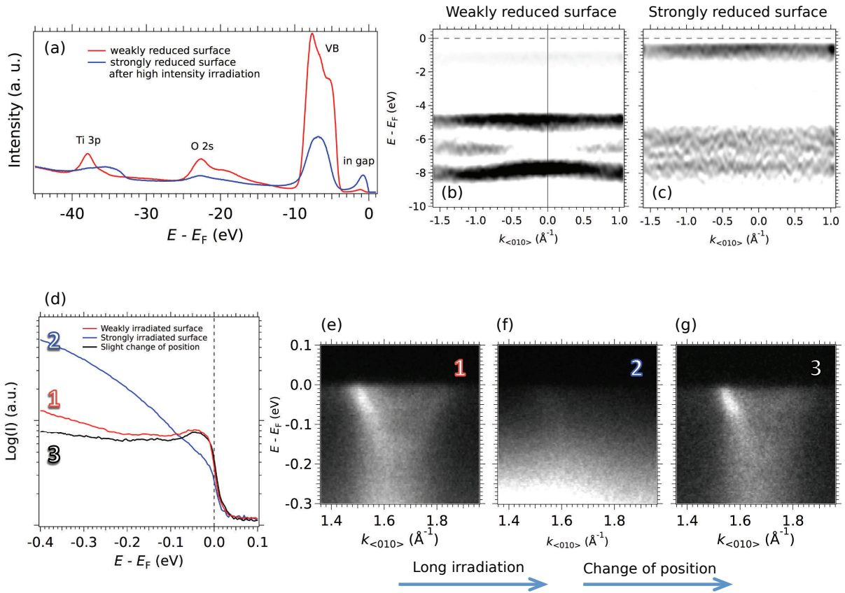
Figure 3.11: (a) Angle-integrated spectra of a cleaved TiO 2 (001) anatase sample measured at h\nu = 100 eV showing the density of states for binding energies between -45 eV and 2 eV. The red curve corresponds to a weakly reduced surface, the blue one to a surface exposed to the intense zero-order light irradiation of the synchrotron. (b, c) Corresponding angle-resolved energy-momentum maps (second energy derivatives, negative values only) zoomed over the valence-band region. While the valence band is dispersive in the crystalline, weakly irradiated surface, it becomes non-dispersive and featureless in the amorphous, strongly irradiated surface. (d) Angle-integrated spectra measured at h\nu = 47 eV (log scale for spectral intensity), showing the tail of the in-gap peak and the intensity at the Fermi level. The red curve (labeled 1) corresponds to a freshly cleaved sample irradiated for a first sweep, the blue curve (labeled 2) to a surface exposed to irradiation for several hours, and the black curve (labeled 3) to the electronic structure after changing the sample position. (e, f, g) Energy-momentum maps measured at h\nu = 47 eV along the \langle 010 \rangle direction. The momentum-integrated curves of these maps corresponds to the data shown in (d) as indicated by the labels 1, 2 and 3. Published in reference [15].
