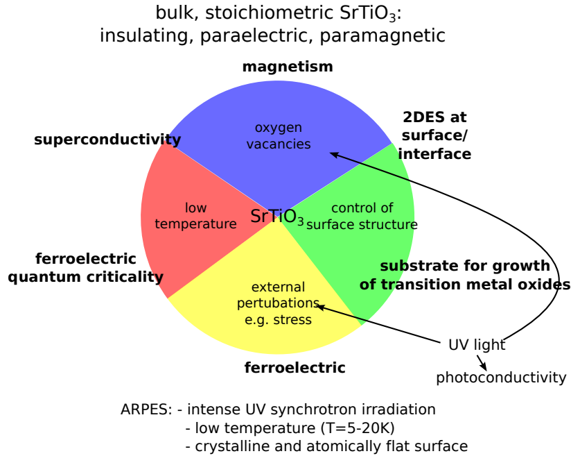
Figure 1.3: Properties of SrTiO 3 depending on presence of oxygen vacancies, temperature, perturbations and the control of the surface structure. Although SrTiO 3 is a paramagnetic, paraelectric and band insulating material in its stoichiometric form, various different properties emerge by slightly disturbing the system. Oxygen vacancies can lead to a 2DES confined at the surface, magnetism and superconductivity at low temperatures. The incipient ferroelectric state can be tuned to a real ferroelectric state by e.g. A-site doping or strain in thin films of SrTiO 3 . UV-light which we used as an experimental probe can create oxygen vacancies or influence the polar order of SrTiO 3 .
