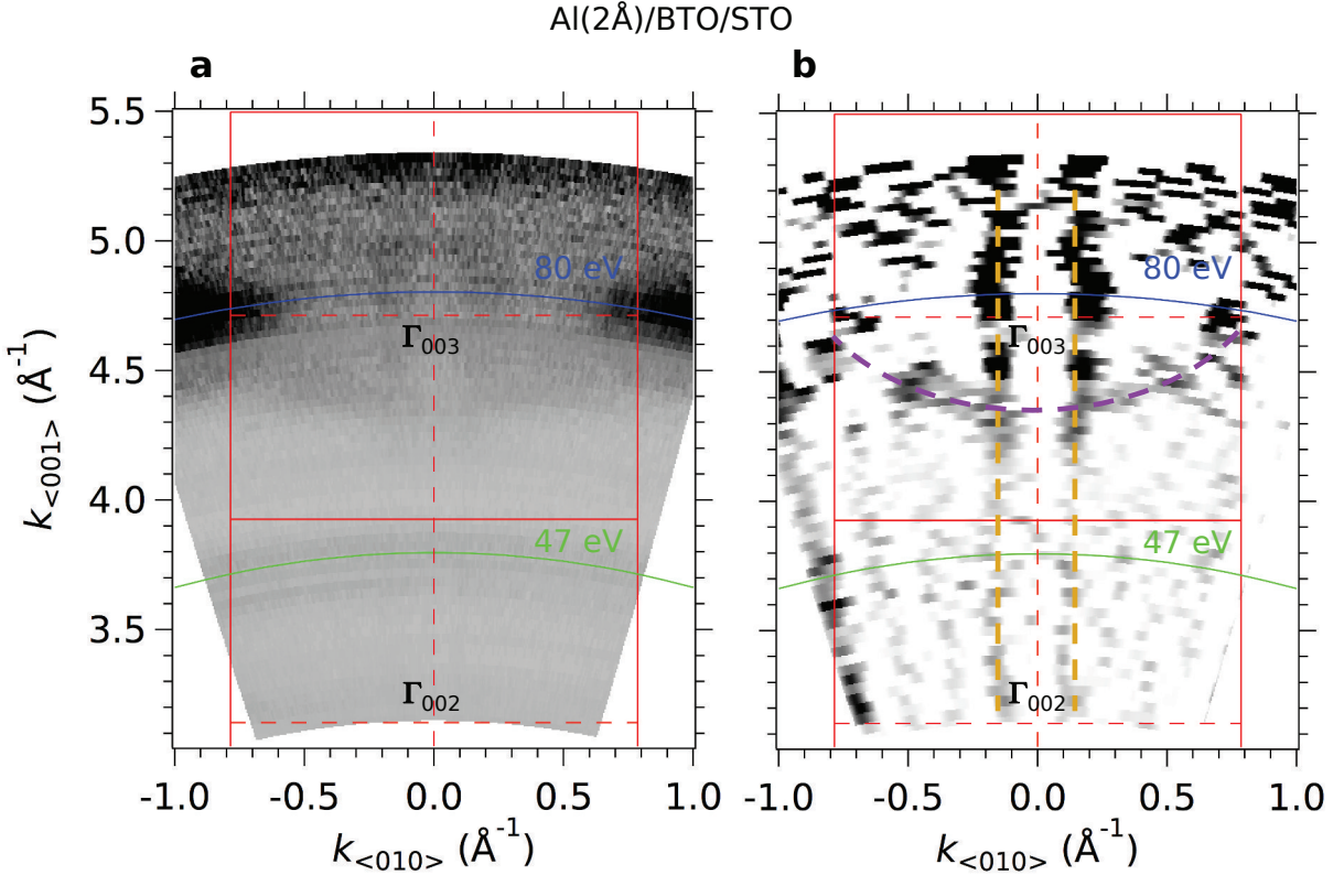
Figure 6.5: 2DES in BaTiO 3 . (a) Raw Fermi surface map at the the Al(2Å)/BaTiO 3 interface in the k_{\langle 001 \rangle} - k_{\langle 010 \rangle} plane, acquired by varying the photon energy in 1 eV steps between h\nu_1 = 30 eV and h\nu_2 = 100 eV using LH photons. To calculate the momentum perpendicular to the surface, we use a free-electron final-state approximation, and set the inner potential to V_0 = 12 eV. The spectral weight was integrated over [E_F - 30, E_F + 5] meV. The red square shows the edges of the \Gamma_{003} bulk Brillouin zone. The blue and green arcs show the spherical cuts in 3D reciprocal space obtained with h\nu = 80 eV and h\nu = 47 eV. Note that the data shown in figures 6.3 and 6.4 were obtained in different Brillouin zones, namely the ones of \Gamma_{103} and \Gamma_{102} . (b) Second derivative (negative values only) of the Fermi surface map in (a). The yellow and purple dashed curves are guides to the eye showing, respectively, the non-dispersive Fermi surface of the light d_{xy} -like states, and the dispersive Fermi surface of the heavy d_{xz/yz} -like states. The measurement was conducted at a temperature of T = 8 K. Published in reference [19].
