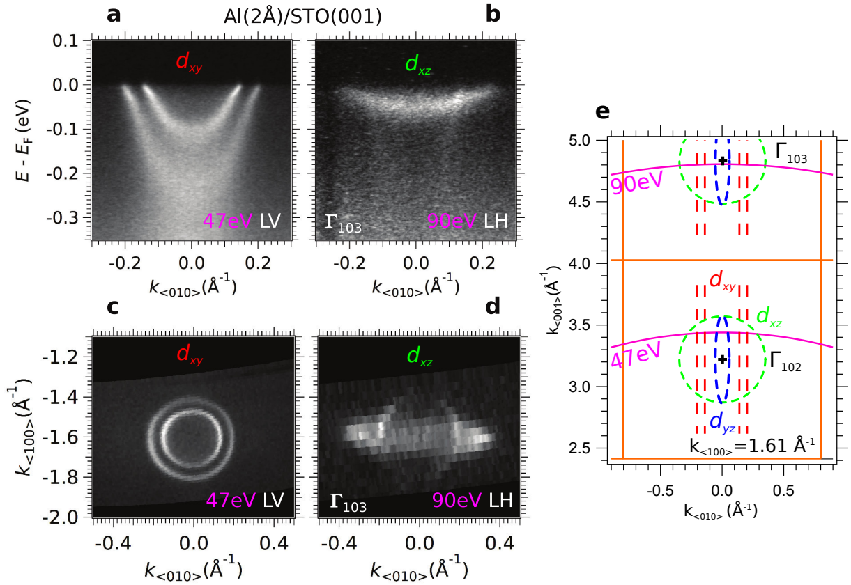
Figure 4.4: (a, b) ARPES energy-momentum intensity maps measured at the Al(2Å)/SrTiO 3 (001) interface prepared in-situ , using respectively 47 eV (LV) and 90 eV (LH) photons. (a) Two d_{xy} subbands with effective mass of m_{xy}^* \approx 0.7 and band bottoms at E_{xy,1} = 223 meV and E_{xy,2} = 110 meV. Using the nomenclature in section 2.2, the mirror plane is the xz plane and thus, only bands of d_{xy} and d_{yz} character have non-zero matrix elements at k_{\langle 010 \rangle} = 0 using LV photons (see table 2.1 on page 31). As shown in (e), h\nu = 47 eV corresponds to position in reciprocal space which are off the bulk \Gamma point. That is why only d_{xy} bands are visible. (b) d_{xz} subband with effective mass of m_{xy}^* \approx 7 and a band bottom at E_{xz} = 50 meV. Only d_{xz} orbitals can be detected at k_{\langle 010 \rangle} = 0 using LH photons given that the photon energy h\nu = 90 eV corresponds or is close to a bulk \Gamma point.
