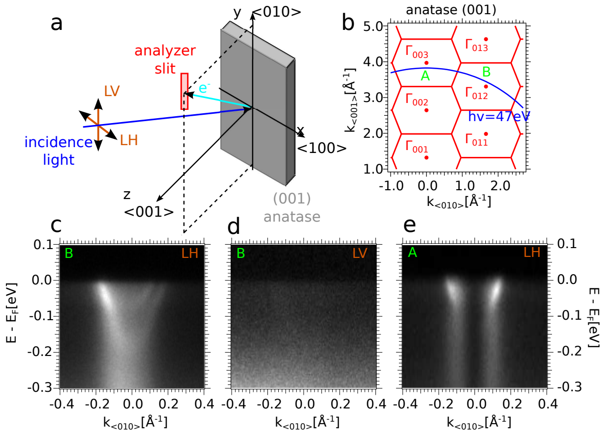
Figure 3.9: (a) Sketch of the experimental ARPES setup. (b) Schematic representation of the reciprocal space of bulk \text{TiO}_2 anatase over several Brillouin zones in the (100) plane. (c) Energy momentum map measured at h\nu = 47 \text{ eV} with linear horizontal light polarization (LH) at the surface of a tilted sample corresponding to position B in reciprocal space in (b). (d) Same as (c) but with linear vertical light polarization (LV). (e) Same as (c) but at normal emission, position A in (b). Published in reference [15].
