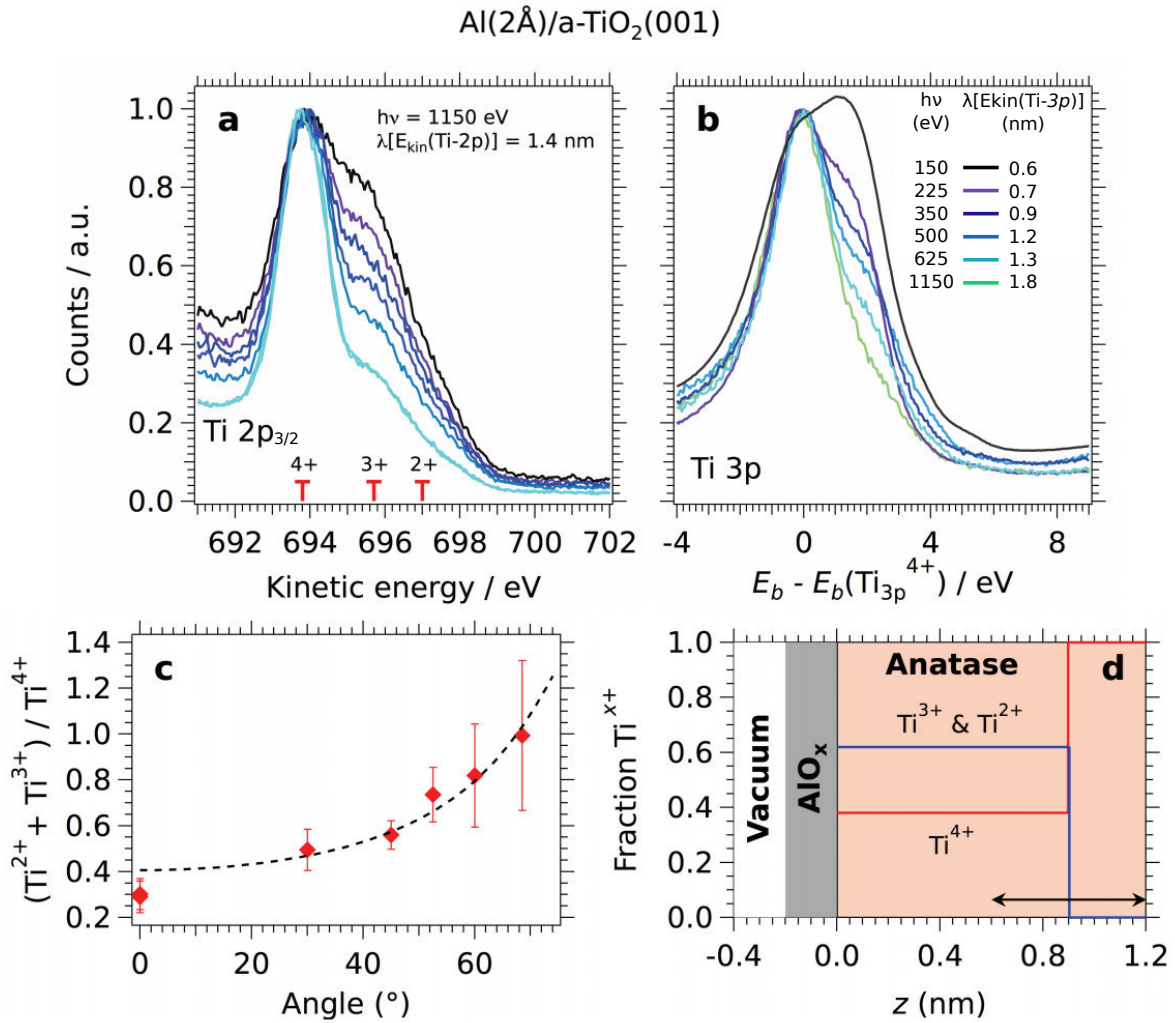
Figure 3.5: (a) XPS of the Ti- 2p_{3/2} core level of Al(2Å)/anatase(001) as a function of emission angle using h\nu = 1150 \text{ eV} photons. At this photon energy, the universal inelastic mean free path of electrons emitted from the Ti- 2p_{3/2} peak corresponds to \lambda[E_{kin}(\text{Ti-}2p)] = 1.4 \text{ nm} according to [114]. The red markers and corresponding error bars indicate the peak positions and uncertainties for the different Ti oxidation state (4+, 3+, and 2+). (b) XPS of the Ti- 3p core level of anatase (001) at normal emission as a function of photon energy. The inelastic mean free path of electrons emitted from the Ti- 3p peak at different photon energies is specified in the inset table. The XPS intensity in panels (a) and (b) is normalized to the Ti 4+ peak. (c) Ratio of intensities, from panel (a), between the Ti 2+ + Ti 3+ shoulder and the Ti 4+ peak as a function of the electron ejection angle. The dashed curve is the best fit to the data assuming a step-like distribution of vacancies over 9 \pm 3 \text{ \AA} below the surface, as schematized in panel (d). (d) Model used for the distribution of the different Ti oxidation states due to oxygen vacancies beneath the AlO x /anatase interface: blue line for Ti 2+ + Ti 3+ , red line for Ti 4+ . The double arrow indicates the error bar in the determination of the vacancy depth distribution. Published in reference [19].
