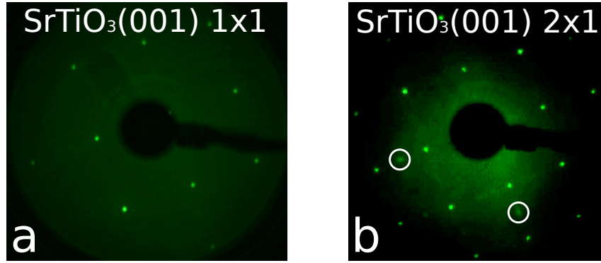
Figure 2.11: (a) LEED image of a unreconstructed \text{SrTiO}_3(001) surface annealed at T=550^\circ\text{C} in UHV. Annealing at higher temperatures can result in a surface reconstruction as the 2 \times 1 reconstruction shown in (b). (b) LEED image of a \text{SrTiO}_3(001) sample annealed at T=700^\circ for approximately 1h. The diffraction spots corresponding to the two domain ( 2 \times 1 ) reconstruction are highlighted by the white circles.
