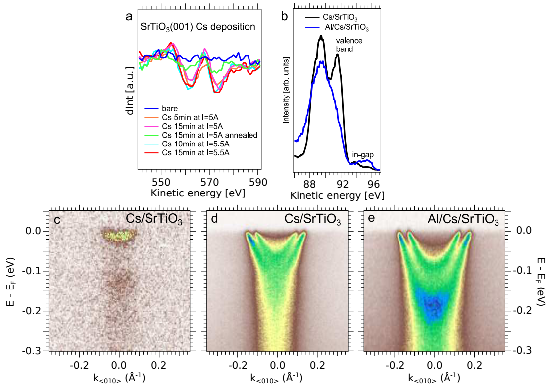
Figure 4.14: (a) Cs-Auger spectra of SrTiO 3 before and after deposition of Cs with various different parameters (duration of deposition and current to the Cs source). The energy of the incident electrons was 2 kV. Independent of the deposition parameters the Cs peak height is identical indicating that maximal one monolayer of Cs can be deposited. (b) Angle-integrated photoemission spectra of valence band and band gap region of the Cs/SrTiO 3 as well as the Al/Cs/SrTiO 3 interface. The different intensities of the in-gap state indicate different concentration of oxygen vacancies in SrTiO 3 close to the interface. (c) - (e) Energy-momentum map close to the Fermi level measured at h\nu = 47 eV ( \Gamma_{102} ) at the SrTiO 3 based interfaces. (c) The lowest electron density is at the Cs/SrTiO 3 interface right after the first exposure of the sample to the synchrotron irradiation. (d) After one to two hours of irradiation, the electron density reaches a saturation value. (e) The deposition of Al acting as oxygen sink further increases the electron density.
