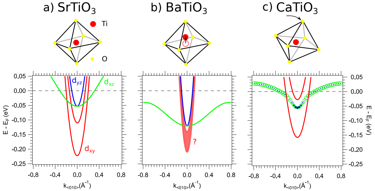
Figure 6.8: Oxygen octahedron in ATiO 3 (A=Sr,Ba,Ca) perovskites and schematic of band dispersion observed in the 2DESs in SrTiO 3 (a), BaTiO 3 (b) and CaTiO 3 (c). The broad red band and the question mark in (b) indicate that the band structure of the d_{xy} band was not determined precisely in BaTiO 3 . The colors of the bands corresponds to different orbital characters. The size of filled and empty markers in (c) represent the fraction of the d_{xz} (green) and the d_{yz} (blue) in the band dispersion.
