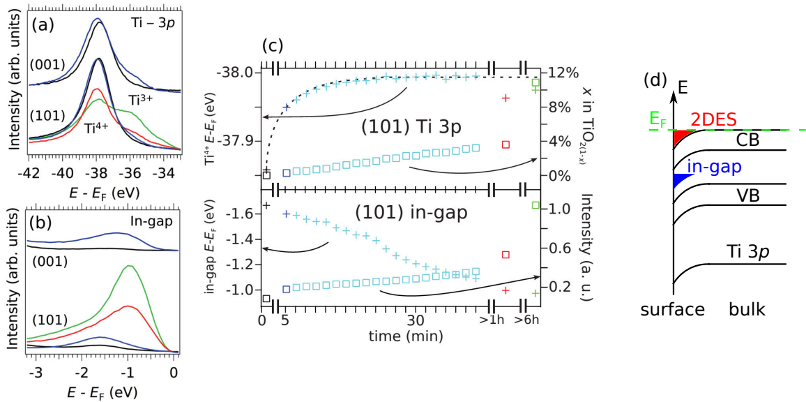
Figure 3.4: Angle integrated spectra of (a) the Ti-3 p peak, and (b) the in-gap state of the anatase TiO 2 (001) and (101) surfaces (upper and lower curves, respectively) measured at h\nu = 100 eV. The black curve was measured shortly after the first light exposure, and the blue, red and green curves at sequentially increasing times. (c) Binding energy of the Ti 4+ peak and concentration of oxygen vacancies (ratio between the Ti 3+ and total Ti-3 p peak area) for different durations of irradiation exposure of the (101) surface (upper panel), and binding energy and intensity of the in-gap state (lower panel). (d) Schematic band alignment along the confinement direction showing the band bending at the surface which confines the 2DES. (a-c) Published in reference [15].
