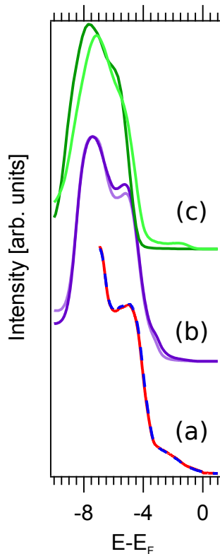
Figure 3.2: Angle-integrated spectra measured at a photon energy of h\nu = 21.2 eV (a) or 100 eV (b,c) at fractured or in situ prepared surfaces of SrTiO 3 (001). (a) No spectral changes are induced by the irradiation because the photon flux or photon energy of He lamp are too low to desorb oxygen from the surface. The blue curve was measured 12 hours after measuring the red curve. (b) The photon flux at the beamline 9B in the HiSOR synchrotron is too low to induce significant changes (no in-gap state). (c) The in-gap state can be created using the much more intense irradiation of 0 th order of the monochromator grating (reflected, polychromatic beam).
