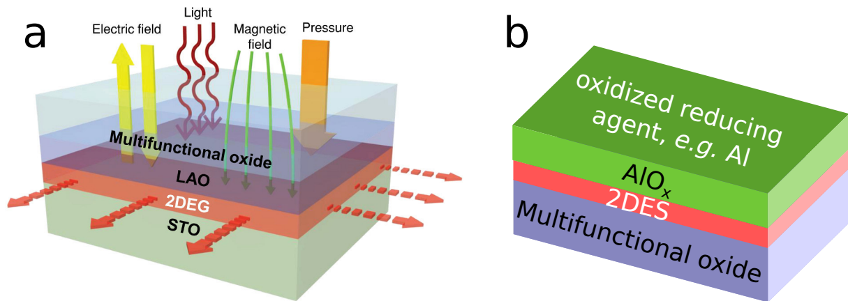
Figure 9.2: (a) Schematic illustration of the functionalization of the 2DES at the \text{LaAlO}_3/\text{SrTiO}_3 interface using epitaxial heterostructuring proposed by Kim et al. [254] (b) Instead of altering the properties of the 2DES at the \text{LaAlO}_3/\text{SrTiO}_3 interface using a multifunctional oxide on top of \text{LaAlO}_3 , we propose to create and control a 2DES in the multifunctional oxide itself using an elementary reducing agent ( e.g. Al).
