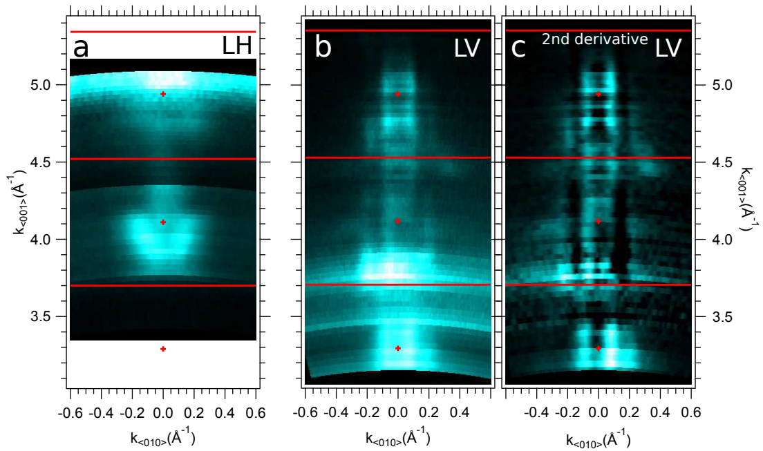
Figure 6.7: 2DES in \text{CaTiO}_3 . (a) Fermi surface map in the k_{(001)} - k_{(010)} plane measured by changing the photon energy between h\nu = 37 eV and h\nu = 90 eV using LH polarization. (b) FS map with photon energies ranging between h\nu = 30 eV and h\nu = 100 eV using LV polarization. (c) Same as (b) but based on 2 nd derivatives of the energy momentum maps. The red lines show the Brillouin zone border of the orthorhombic lattice and the red markers correspond to \Gamma points of the reciprocal lattice. All measurements were conducted at temperatures ranging between T = 7 - 20 K.
