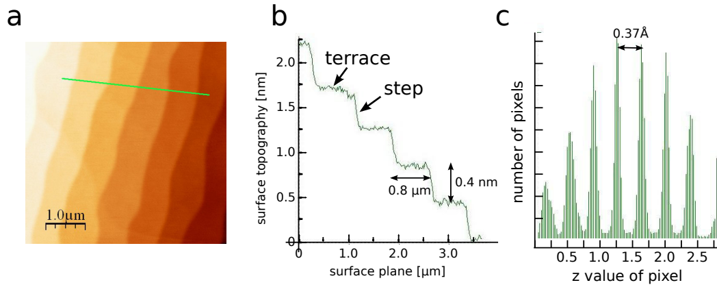
Figure 2.10: (a) Atomic force microscopy (AFM) image of a chemically and thermally prepared \text{SrTiO}_3(001) surface. A step-and-terrace structured surface is visible. (b) The profile of the surface along the green line in (a). The numbers indicate the width of one terrace and respectively, the step height. (c) The histogram of the AFM image helps to approximate the step height.
