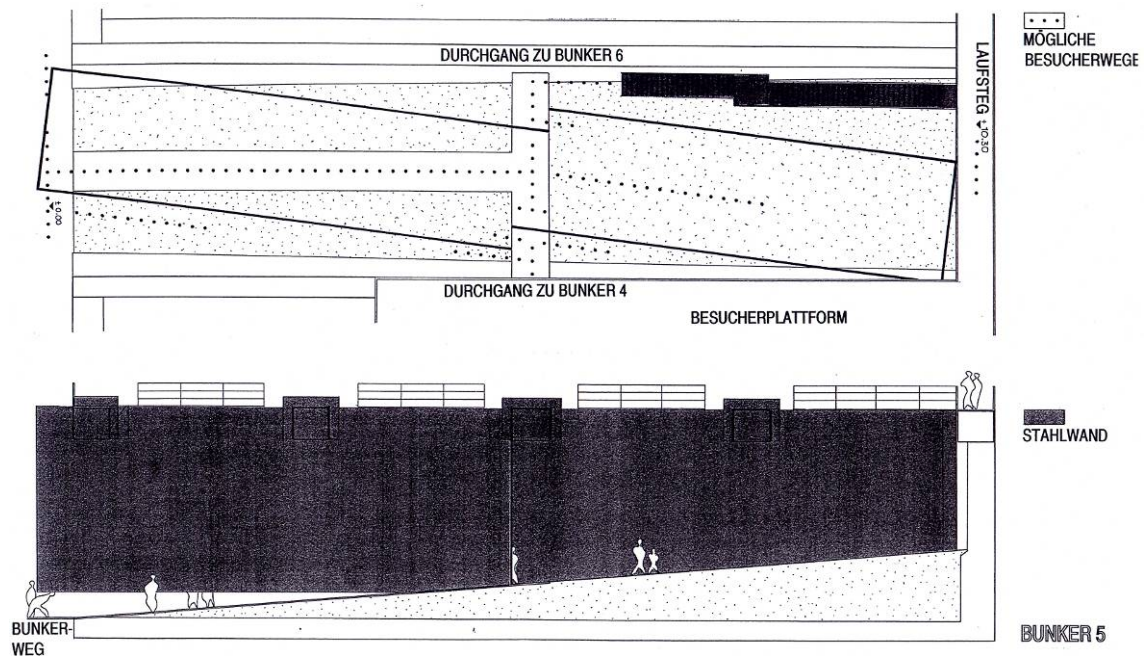
Figure 17 - Pit Koker, floor plan for bunker project
