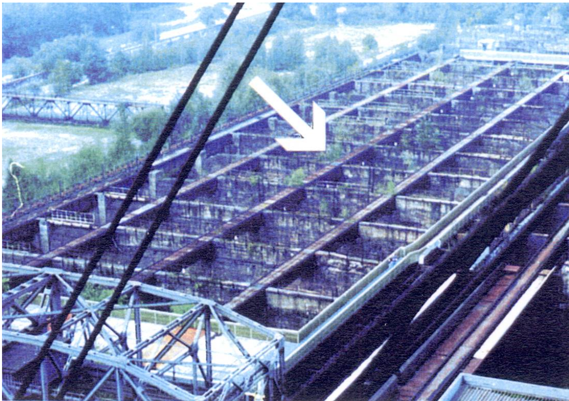
Figure 16 - Stäbler, series of industrial coal bunkers
