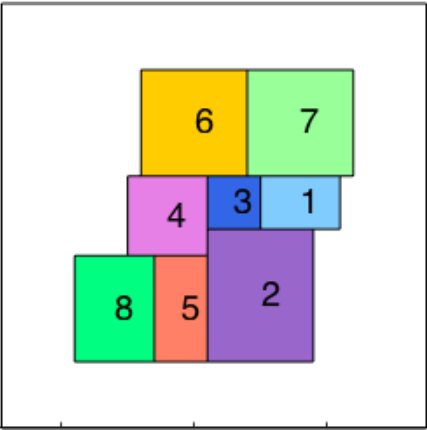
Type I: 8 block problem (191.5) time = 264.5751s
