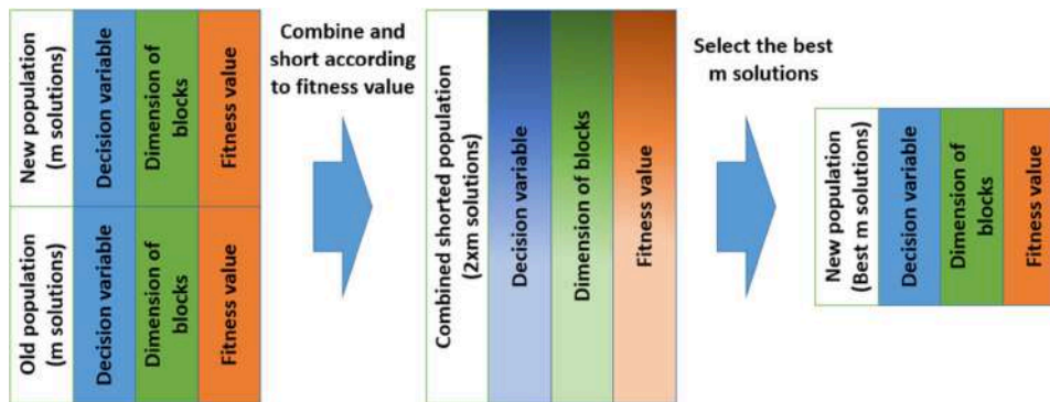
Figure 5.12. Elitism Operator
