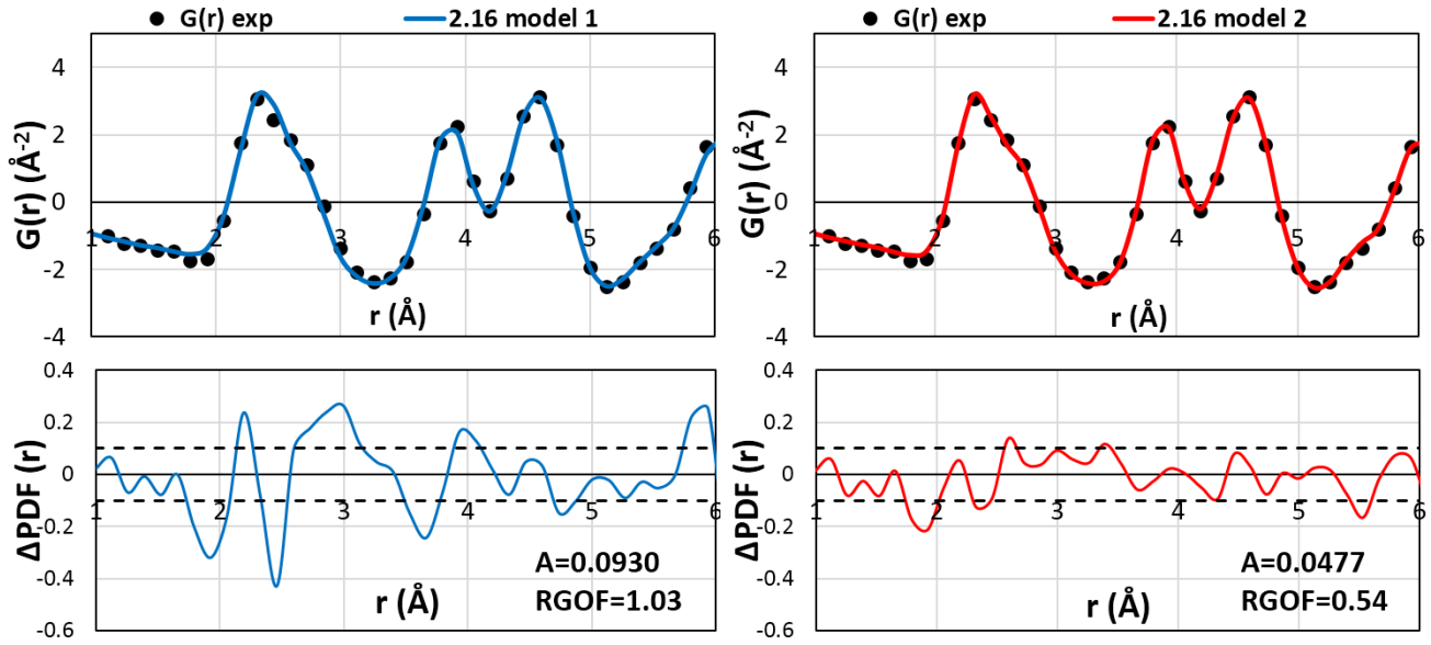
Figure 3.12: PDF data for UO 2.16 (black open circles) up to 6 Å at 900 °C and fourfold-cell model results refined using the PDFgui. On the left: Model 1; on the right: Model 2; The black dashed lines indicate the experimental uncertainties.
