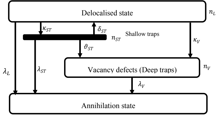
Figure 2.24: Positron trapping in various states (Krause-Rehberg and Leipner, 1999b).
