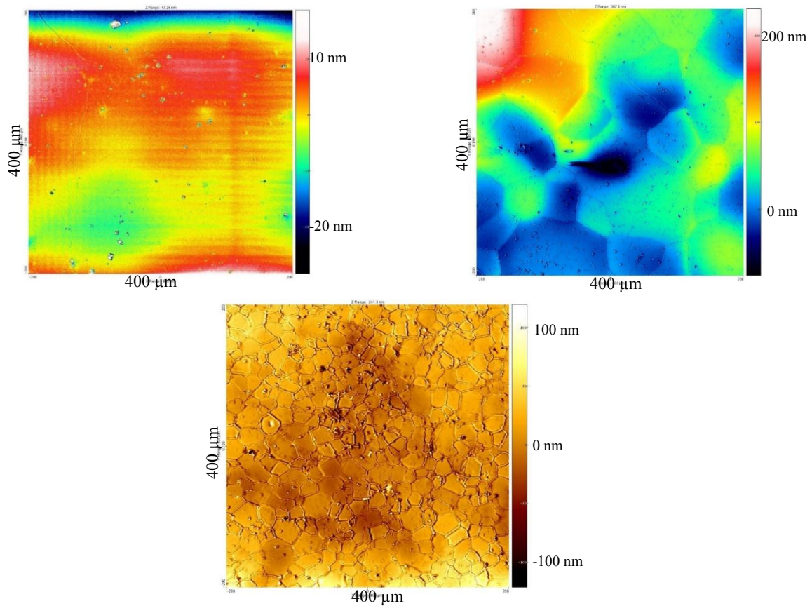
Figure 2.5: 400×400 \mu\text{m}^2 chromatic confocal microscope images of samples: top left – single-crystal \text{UO}_2 following annealing at 1700 °C; top right – Cr-doped \text{UO}_2 following the last polishing stage; bottom – poly-crystal \text{UO}_2 following annealing at 1700 °C.
