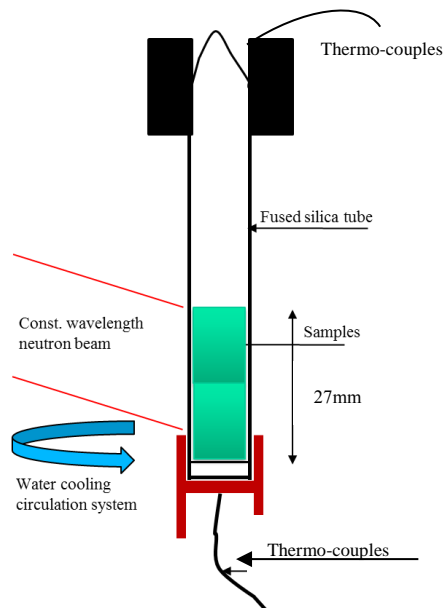
b) Schematic diagram illustrative of sample and container inside the furnace.
