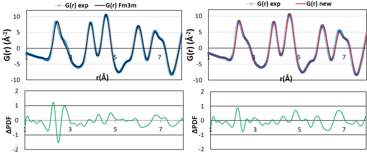
Figure 3.10: Experimental PDF (blue circles) of \text{UO}_2 at 900 °C refined assuming a Fm\bar{3}m structure (black line) and oxygen anharmonic behaviour (red line) up to 8 \text{\AA} ; the difference between experimental data and refined results is illustrated in green.
