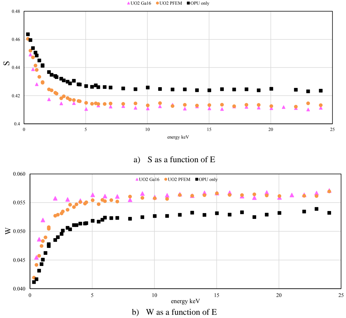
Figure 4.4: Low and high momentum distribution fractions of \text{UO}_2 samples at 300 K as a function of positron beam energy; Squares represent as-polished \text{UO}_2 ; the triangles represent the polished and subsequently annealed sample in a humidified \text{Ar}/\text{H}_2 gas mixture; and the circles represent the polished and subsequently annealed sample in a dry \text{Ar}/\text{H}_2 gas mixture.
