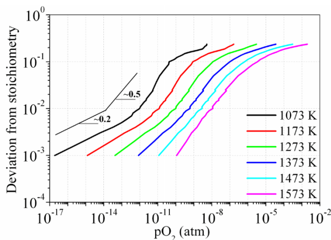
Figure 1.3: Dependence of deviation-from-stoichiometry upon oxygen partial pressure and temperature for hyper-stoichiometric \text{UO}_{2+x} (Perron, 1968).
