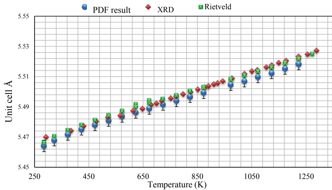
a) Lattice parameter as a function of temperature determined by PDF and Rietveld modelling in comparison to XRD results taken from (Ruello, 2001).
