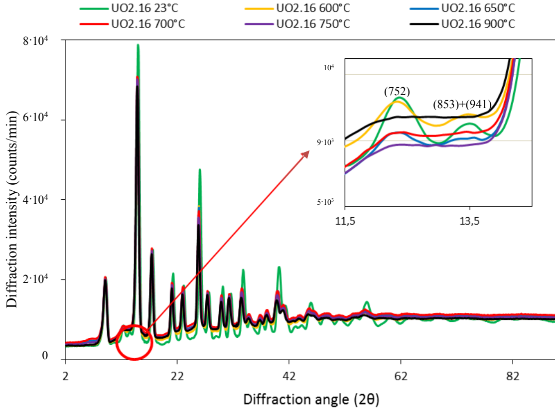
b) Diffraction spectra of \text{UO}_{2.16} obtained at 23 °C, 600 °C, 650 °C, 700 °C, 750 °C, and 900 °C; the inset shows the diffractogram between 11.5 ° and 14 °.
