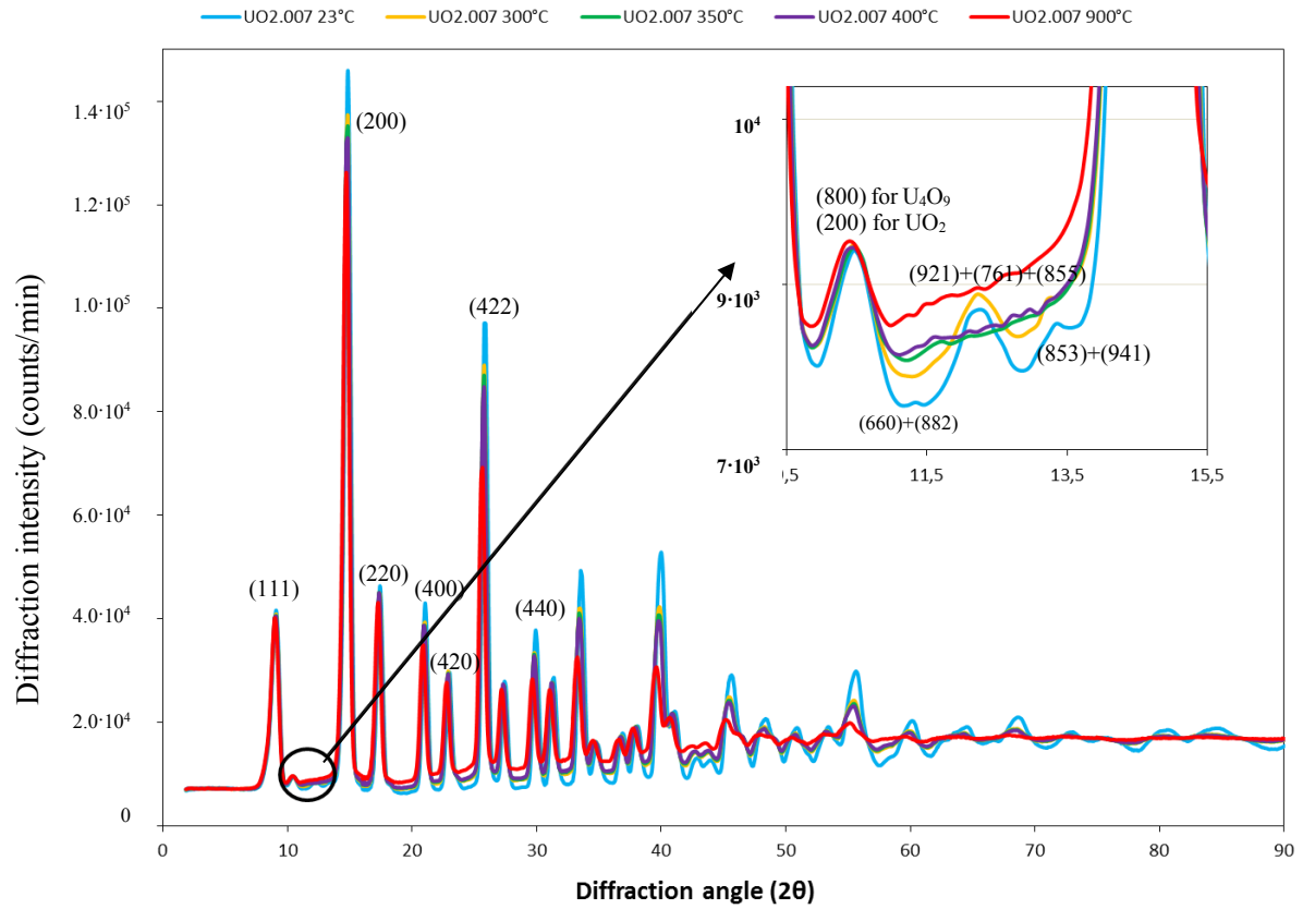
a) Powder diffraction spectra of \text{UO}_{2.007} obtained at 23 °C, 300 °C, 350 °C, 400 °C, and 900 °C; the inset shows the diffractogram at 2\theta between 9.5° and 15.5°.
