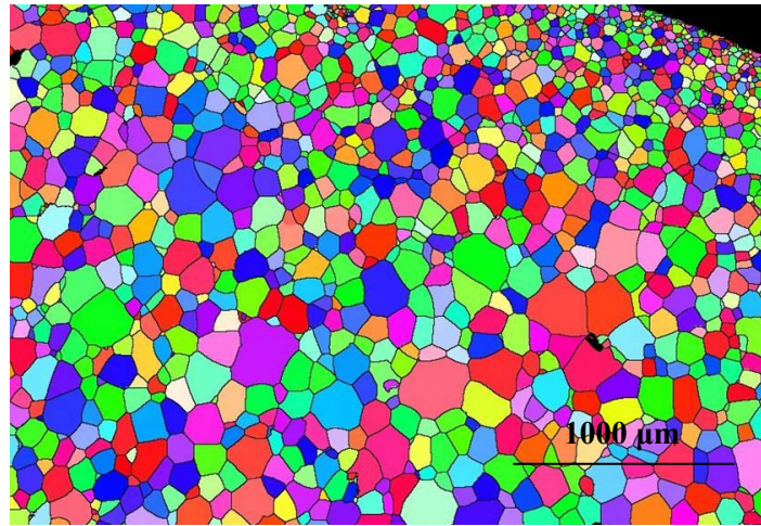
b) EBSD map of a Cr-doped UO 2 pellet cross-section. Colours correspond to different grain orientations.
