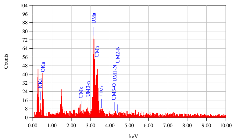
b) EDX analysis of a poly-crystalline \text{UO}_2 sample following the nitrate deposit to low-temperature annealing: the relative concentrations: N – 19%; O – 36%; U – 45%.
