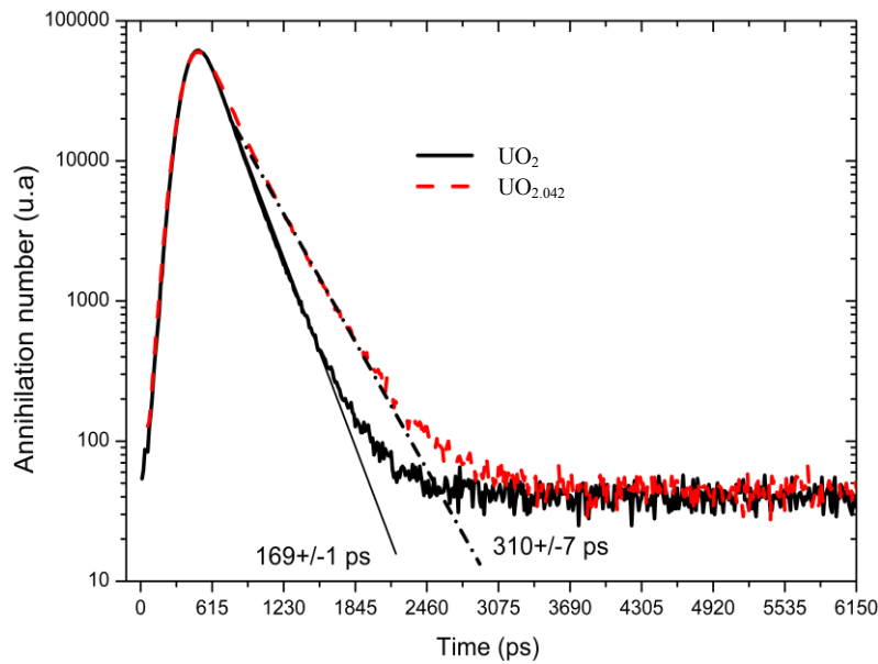
Figure 2.23: Two raw positron lifetime spectra measured in \text{UO}_2 and \text{UO}_{2.04} at room temperature (300 K).
