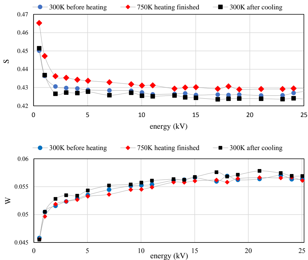
a) S(E) and W(E) of \text{UO}_{2.042} measured at 300 K, then heated to 750 K and then cooled to 300 K again.
