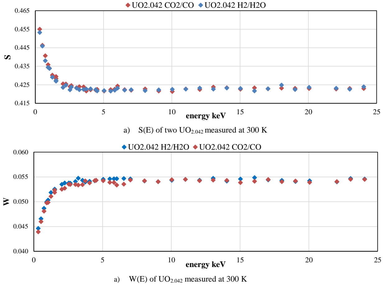
Figure 4.6: Positron momentum distribution fractions of two UO_{2.042} prepared under different gas equilibria
