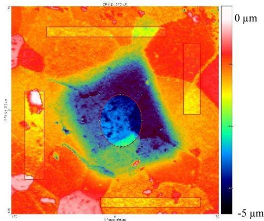
c) Colour coded image of one crater on a Chromium-doped UO 2
