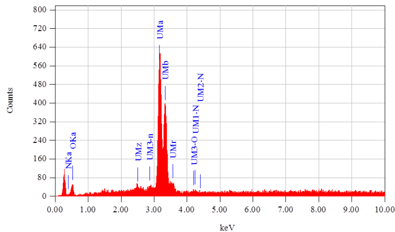
a) EDX analysis of an as-prepared poly-crystalline \text{UO}_2 sample prior to the nitrate deposit: the relative concentrations of three elements of interest are: N – 5 %; O – 16%; U – 79%.
