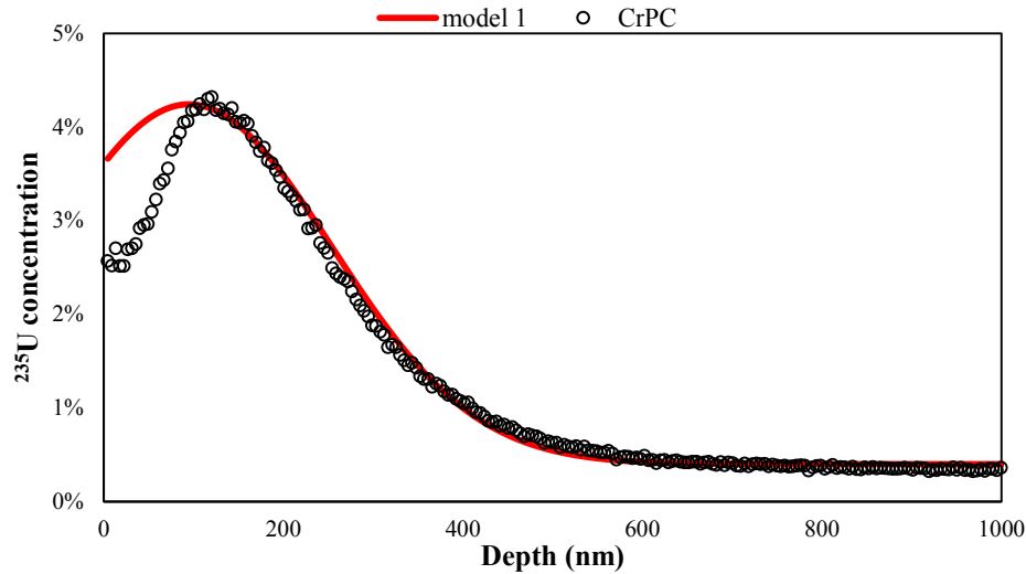
Figure 5.11: Depth profile for the Cr-doped poly-crystal annealed at 1500 °C and slightly oxidizing environment and corresponding modelling results in colour.
