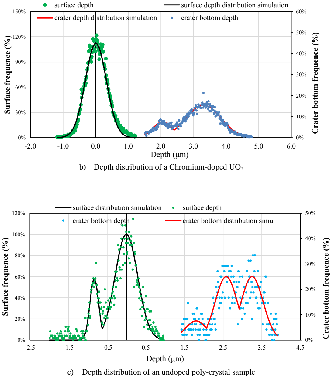
Figure 5.2: Examples of altitude distributions at the bottom and surface of craters a) undoped single-crystal, b) Chromium-doped poly-crystal and c) undoped poly-crystal; blue full circles correspond to the crater bottom and green circles correspond to the sample surface; black and red lines are their respective analytical Gaussian distributions.
