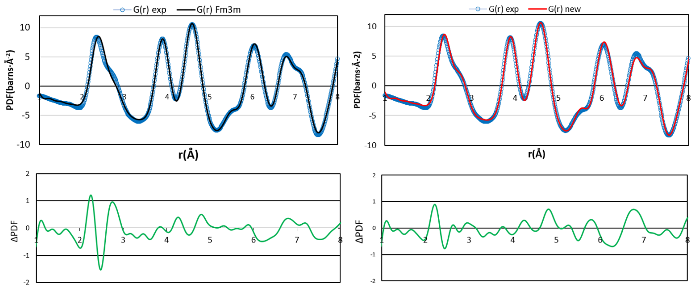
Figure 3.10: Experimental PDF (blue circles) of \text{UO}_2 at 900 °C refined assuming a Fm\bar{3}m structure (black line) and oxygen anharmonic behaviour (red line) up to 8 Å; the difference between experimental data and refined results is illustrated in green.
