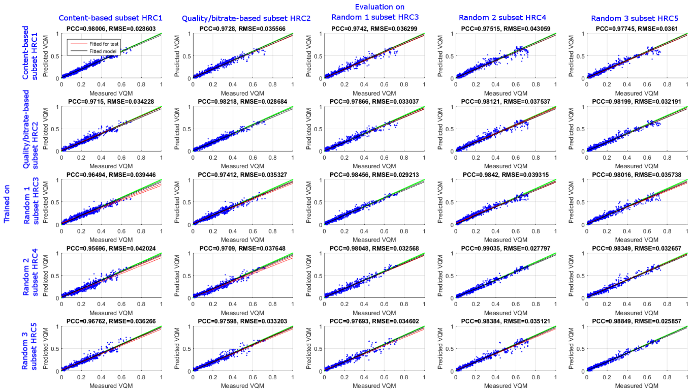
Figure 12.16 – The PCC and the RMSE for the 25 experiments of bitstream-based model. Rows: the different training models that are trained using HRC_1, HRC_2, HRC_3, HRC_4, and HRC_5 . Columns: the test data for each model, from the left, HRC_1, HRC_2, HRC_3, HRC_4, and HRC_5 . The green line is the reference ( y = x ).
