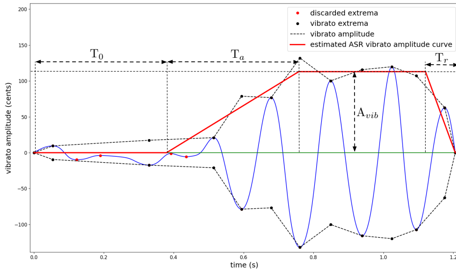
FIGURE 5.10: Vibrato parameters estimation. The vibrato is centered around 0. Then extrema are found for each half cycle. Finally, a continuous amplitude envelope is obtained by linearly interpolating the extrema, to which the ASR envelope is fit.
