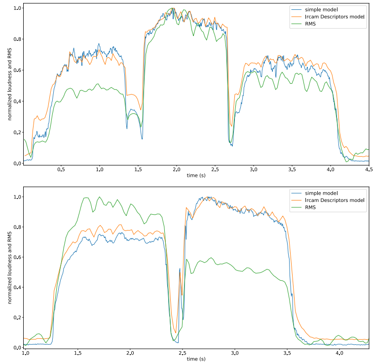
FIGURE 6.10: Comparison of the normalized loudness computed with our loudness model and Zwicker's model, and the normalized short-term RMS, for 2 sounds of the RT database
