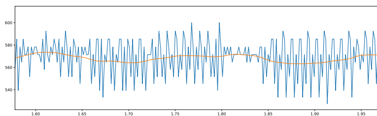
FIGURE 6.24: Jitter extract showing the local f_0 values for individual glottal cycles and the low-passed f_0
