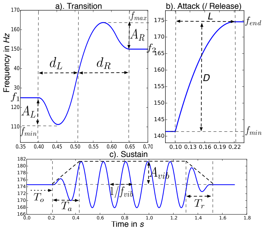
FIGURE 4.8: f_0 model parameters
