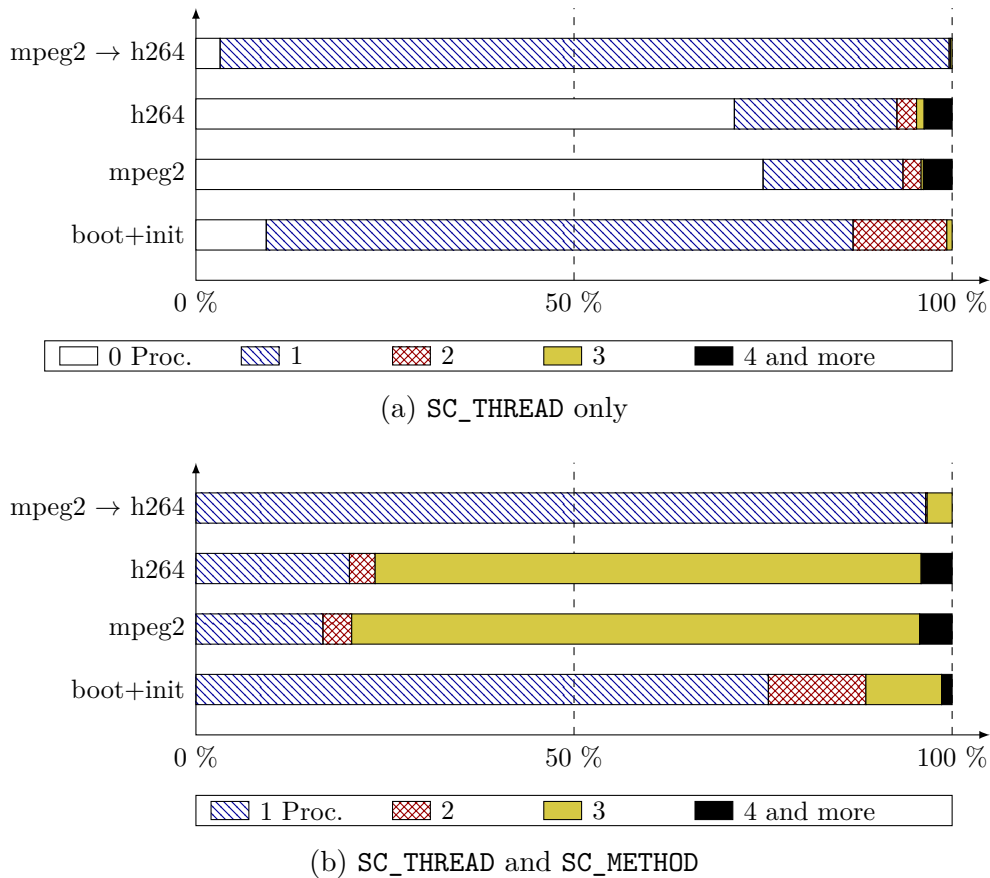
Figure 3.15: Partitioning of delta cycles, per number of runnable processes, for four different test cases, with optimized time picking within time ranges.
