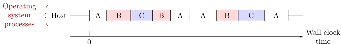
Figure 4.4: Possible execution of this simulation in a sequential simulator such as the reference implementation of SystemC.
