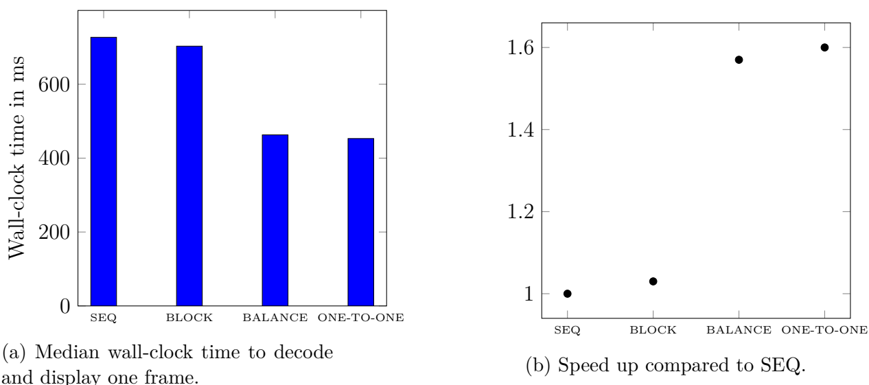
Figure 6.14: Wall-clock time to decode and display one frame of an MJPEG stream, in colors, of a resolution of 1920 \times 800 .
