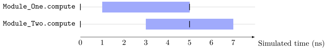
Figure 3.13: Execution diagrams of two processes using loose timing, for two different time choice policies: a random value (a) and a value which maximizes the number of runnable processes (b) in the next cycle.
