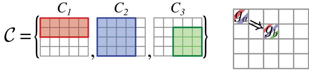
Figure 4.14: Cell g_a implies g_b , or reciprocally g_b is redundant to g_a (right) for given problem instance (left)
