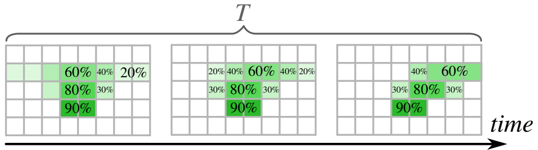
Figure 4.30: Dwell detection probability on the detection grid along the time axis under random radar movement
