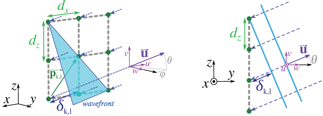
Figure 1.11: Wavefront reception
