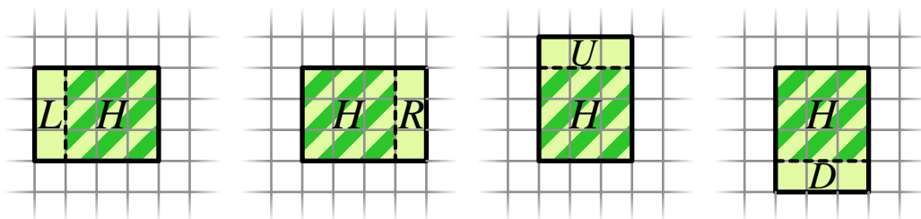
Figure 4.12: The four direct candidate rectangles L , R , U , D for finding a domination cover over rectangle H
