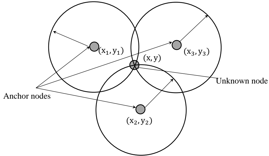
Figure 2.12: Trilateration
