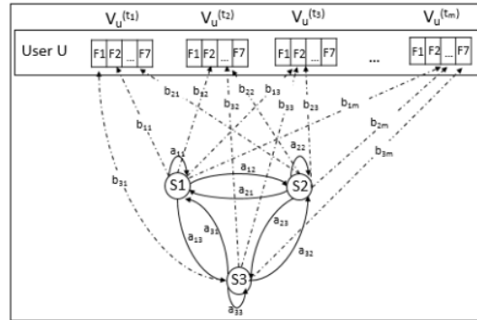
FIGURE 4.5: Temporal representation of user behavior during an event using a 3-state ergodic HMM (Bizid et al., 2015)
