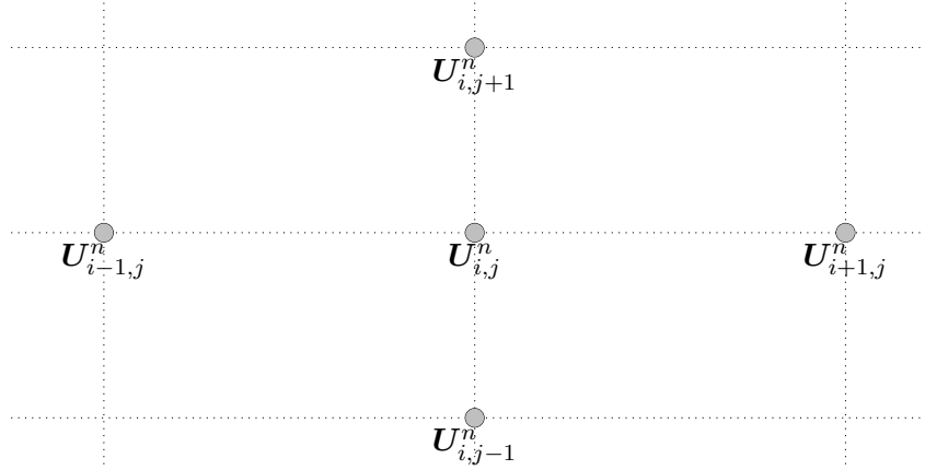
Figure I.1 – Space discretization for centered finite difference schemes on a Cartesian grid
