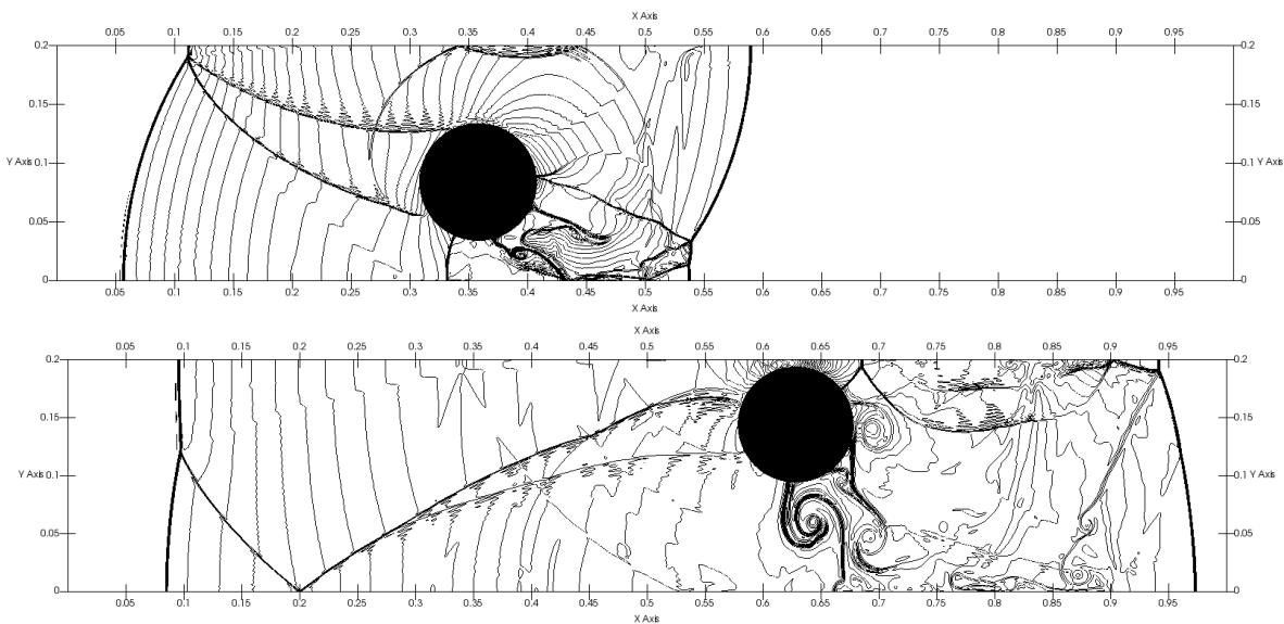
Figure 2 – Rigid-body and compressible fluid coupling. The cylinder is lift off by an incoming shock wave. In return, the shock wave is reflected on the cylinder, and the fluid is displaced by the structure. Complex structures are developed due to the reflection on the top and bottom channel as well as the rigid cylinder. 60 contours are displayed representing fluid density from 0 to 12 at times t=0.14 (top) and t=0.255 (bottom) for the third order scheme, \Delta x = \Delta y = 6.25 \times 10^{-4} .
