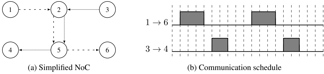
Figure 5.2: Example of application of the Rule 2 of the execution model on simplified NoC with 2 communications competing for a shared NoC resource ② → ⑤
