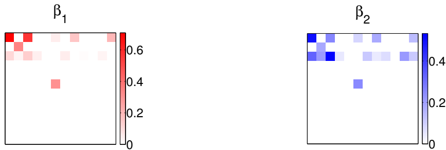
Figure 5.14: Regression matrix in each cluster for the model with 2 clusters
