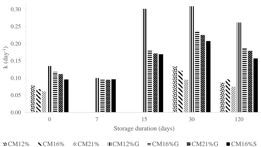
Figure 4-11 – Rate coefficient ( k ) of BMP assays over storage time. Standard deviations are not presented as differences among triplicates were negligible.
