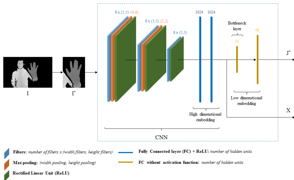
Figure 5.4 – Architecture of the CNN for hand shape and posture extraction using prior enforcement. The model takes as input a cropped depth image I^* around the hand. It uses a CNN architecture to map this image to a high-dimensional space vector X , lying in \mathbb{R}^{1024} . The latter contains large, global and local information about the hand shape. Follows a “bottleneck” layer with a smaller size than the desired output to model the physical constraints over the hand topology. The network finally outputs hand skeletal features J^* centered around the center of mass of the original hand depth image and hand shape features X .
