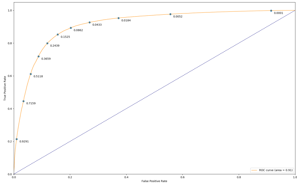
Figure 5.26 – The ROC curve using our framework on the Online DHG dataset. We obtained an Area Under the Curve equal to 0.91.
