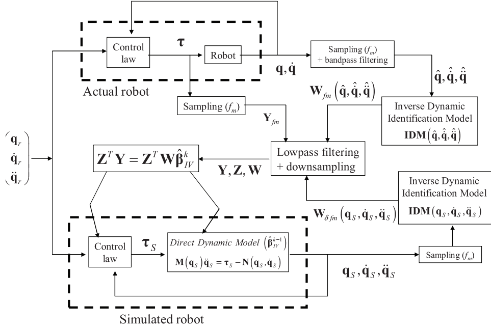
Fig. 4. Scheme of the IDIM-IV identification method.
