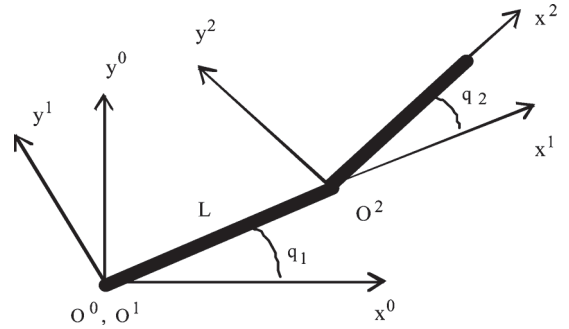
Fig. 9. DHM frames of the scara robot.
