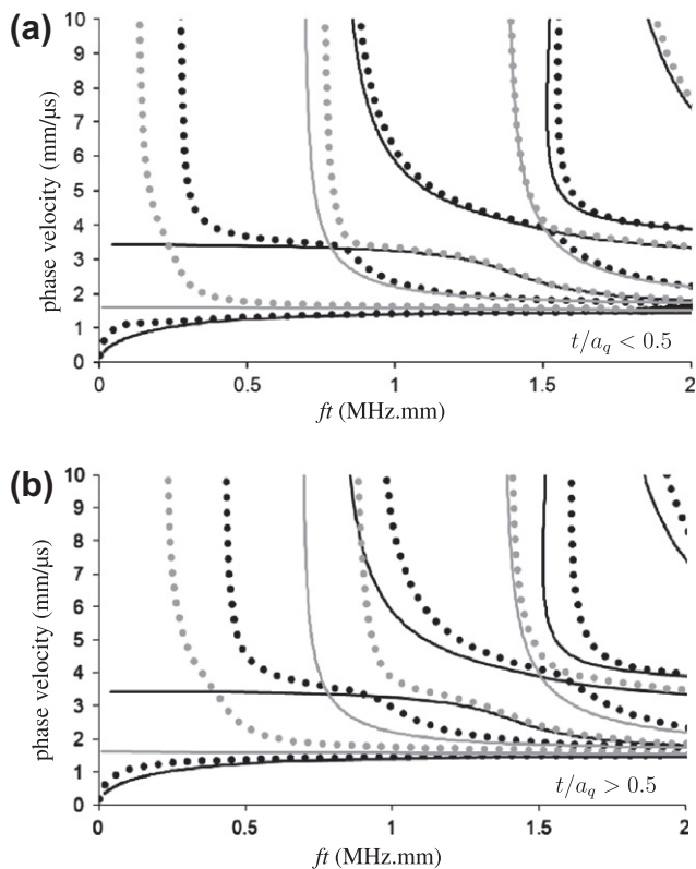
Fig. 8. Influence of the ratio t/a_q for a tube with bone properties (Table 2). The SH modes (grey lines) and Lamb's modes (black lines) are compared with the flexural modes F(1,2m) (grey points) and F(1,2m-1) (black points) with m = 1, 2, 3, 4 .
