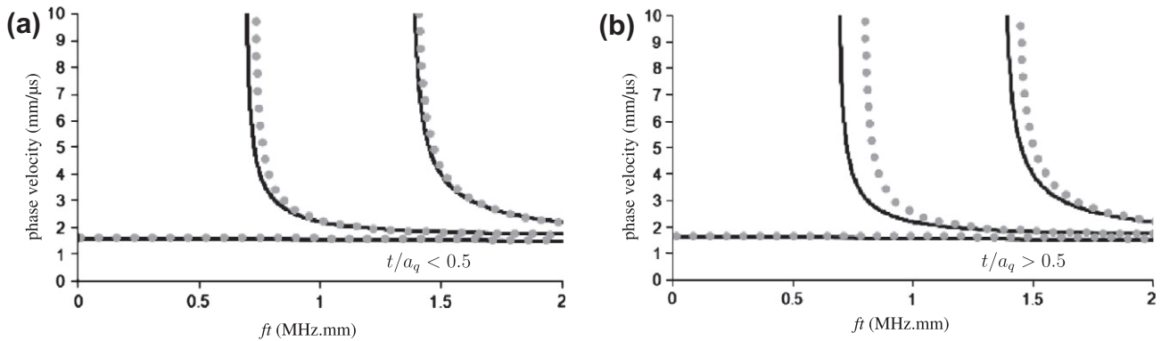
Fig. 7. Influence of the ratio t/a_q for a tube with bone properties (Table 2). The SH modes (black lines) are compared with the torsional modes (grey circles).
