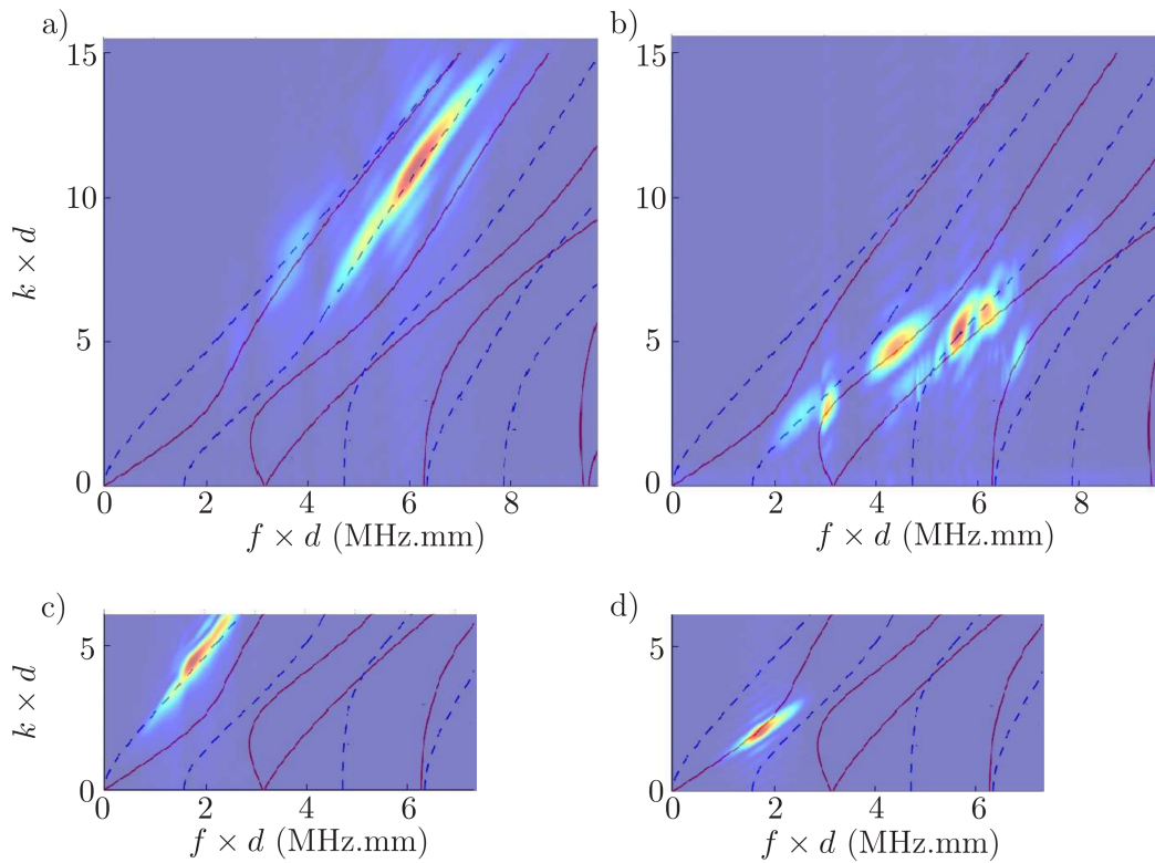
FIGURE 1.4 – Dispersion curves : wave number-thickness product ( k \times d ) function of frequency-thickness product ( f \times d ). a) 5mm-thick aluminium plate, incidence angle of 28^\circ : A_1 mode. b) 5mm-thick aluminium plate, incidence angle of 12^\circ : S_1 and A_2 modes. c) 2mm-thick aluminium plate, incidence angle of 37^\circ : A_0 mode. d) 2mm-thick aluminium plate, incidence angle of 12^\circ : S_0 mode.
