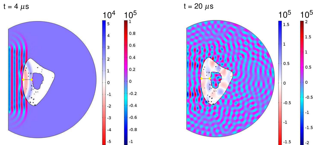
FIGURE 1.15 – Acoustic pressure and interstitial fluid pressure (Pa). The pressure gradient of the interstitial fluid is evaluated between the 2 yellow dots.
