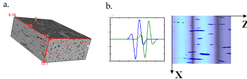
FIGURE 1.1 – Simulation of plane wave propagation (b) through a reconstructed block (a).
