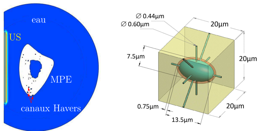
FIGURE 1.14 – Models with mesoscopic (left) and microscopic scales (right). MPE : Poroelastic matrix.
