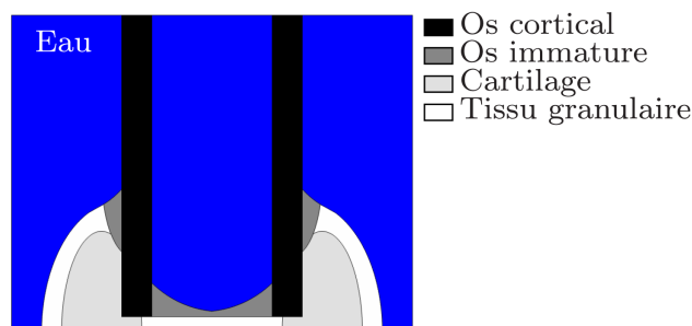
FIGURE 2.2 – Geometry and composition of the bone callus.
