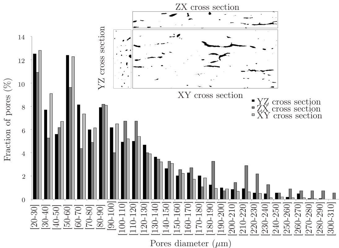
FIGURE 1.5 – Pore diameter distribution along the 3 directions of space for a parallelepipedic sample of adult radius.
