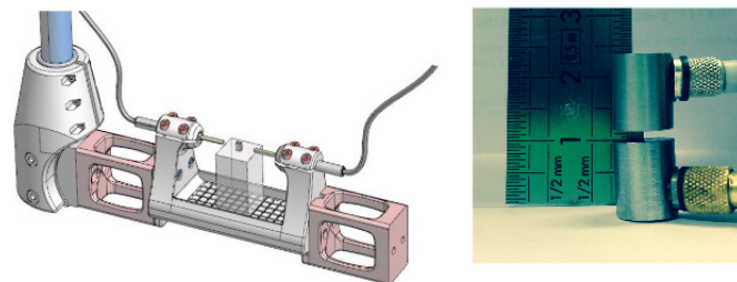
FIGURE 1.8 – Experimental set-ups for ultrasound characterization of millimetric bone samples.
