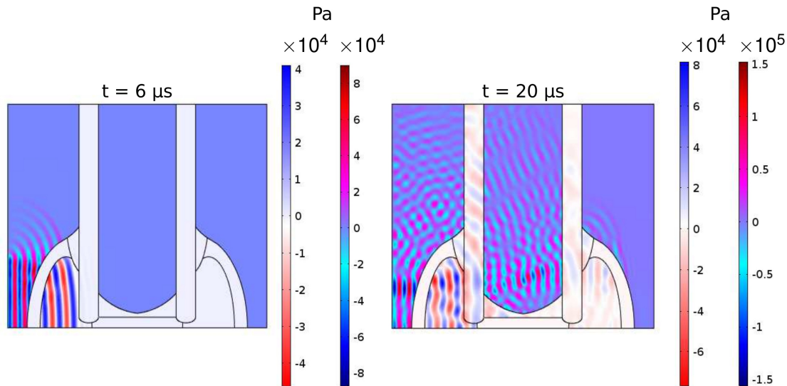
FIGURE 2.3 – Propagation of US waves in the bone callus.
