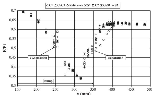
Fig. 6 Wall pressure distributions for steady shock wave configuration without control and with VG devices
