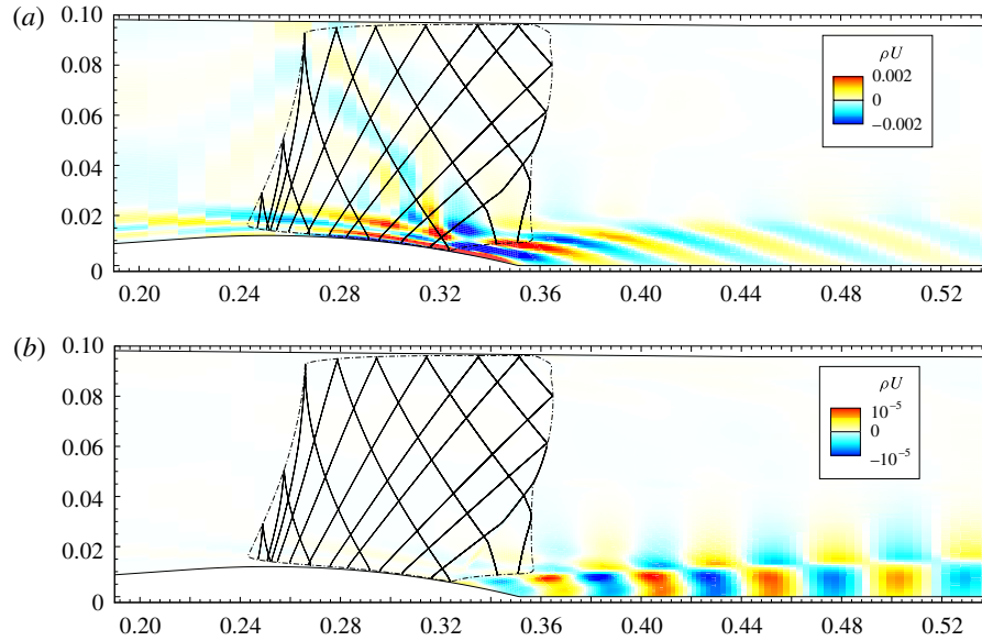
FIGURE 19. (Colour online) Real part of the optimal forcing and associated response at f=4000 Hz. Sonic line (dash-dotted) and characteristics (solid) superimposed. (a) Optimal forcing; (b) optimal response.
