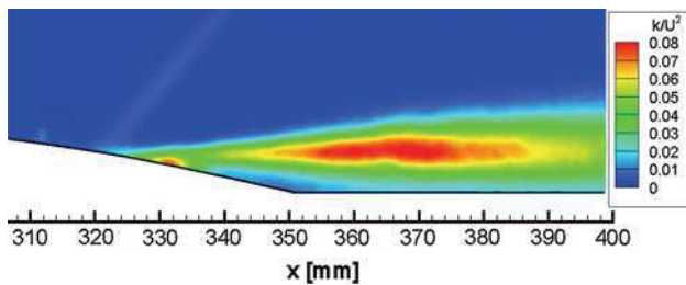
Fig. 10 Evolution of the 2D turbulent kinetic energy k normalized with U_\infty^2
