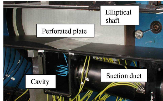
Fig. 1. Photograph of the test set-up with control devices.
