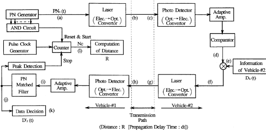
FIGURE 2.25: Block diagram of the boomerang system [110].
