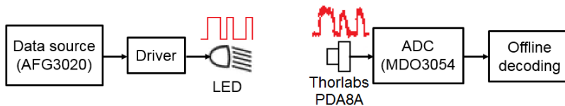
FIGURE 5.22: Emitter and receiver structures used for the VLC experiments with large clock rates.
