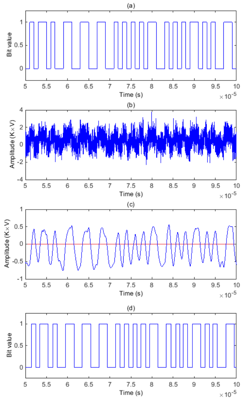
FIGURE 4.22: (a) Data signal transmitted m_e' , (b) signal received m_p with AWGN of SNR = 3 dB, before processing and (c) after filtering with two 2nd order Butterworth filters of respectively low-pass cut-off frequency 500 kHz and high-pass cut-off frequency 5 kHz (blue curve) and hysteresis triggering (dotted and plain red lines), (d) signal d_r reconstructed by triggering.
