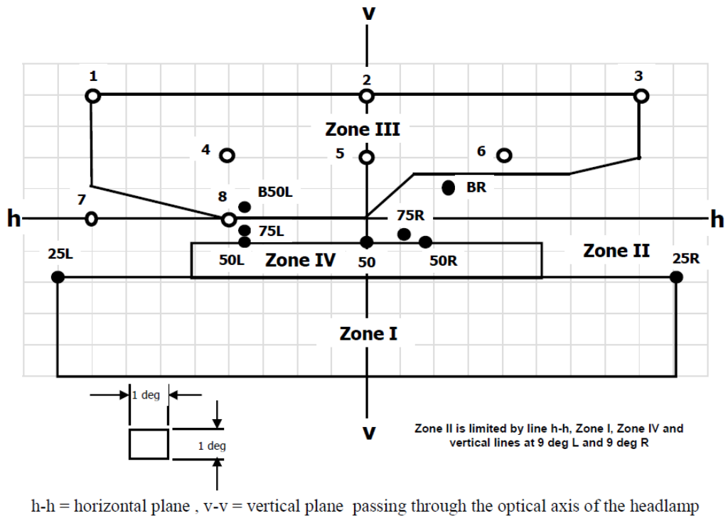
FIGURE A.4: Luminous intensity distribution required for every headlamps in low-beam mode by the ECE R112 regulation [87].
