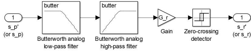
FIGURE 4.4: Details on the signal reconstruction blocks ‘Rx LV’ and ‘Rx FV’ of the VLR.
