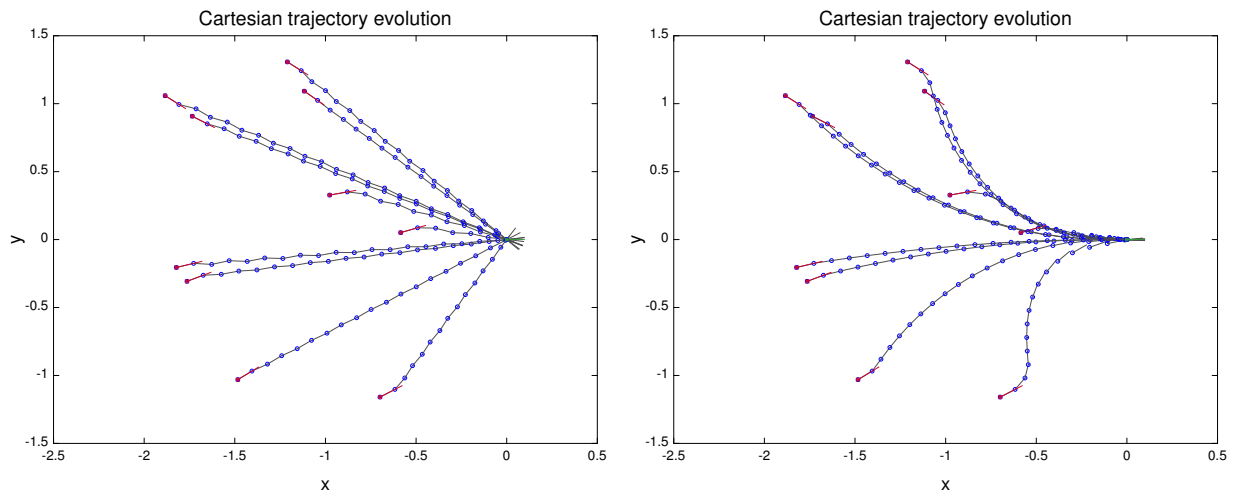
Figure 5.2 – Top view simulation of the Cartesian trajectory followed by the agent. The blue circumferences represent the position and the gray trajectories represent the heading direction. In red the initial configuration, in green the desired configuration. Distances are expressed in meters. On the left the Fajen & Warren description is presented, notice that the final orientation of the body is variable since only the object beating is observed. On the right the HMW proposal is depicted.
