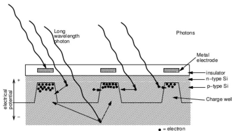
Figure 3.4 – Photosite charge wells and incident photons (Corke [53]). Silicon is more transparent at long wavelengths such that photons may generate electrons deeper within the substrate. This introduces cross-talk between pixels, where the pixel values are not truly independent spatial samples of incident illumination.
