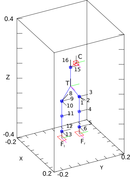
Figure 4.12 – Geometrical model of the robot Nao. Distances are expressed in m. The orientation of the z-axis are projected in black along the structure. For the base frame T and the effector frames C , F_l , and F_r , the x- and y-axis are also plotted in magenta and green respectively. The active joints are numerated and represented by blue boxes. The effectors are represented in red.
