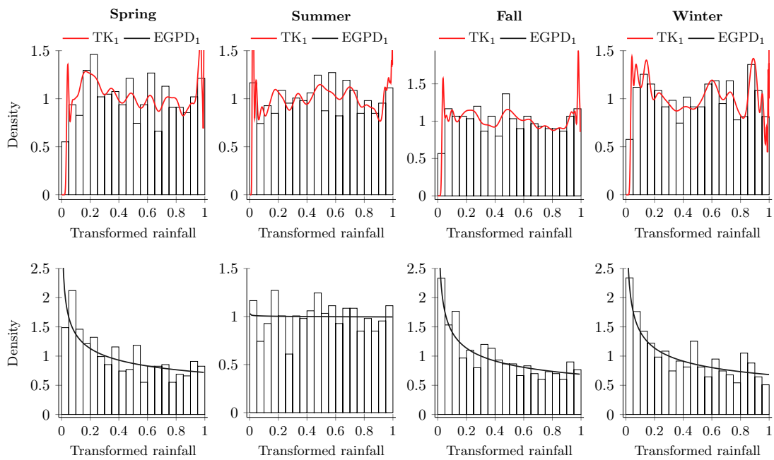
Figure 2.2.10: Histograms with fitted densities of the transformed data U = F_{EGPD_1}(X) and V = H_\xi(X) , for, respectively, TK_1 and EGPD_1 models at Durance station, for each season
