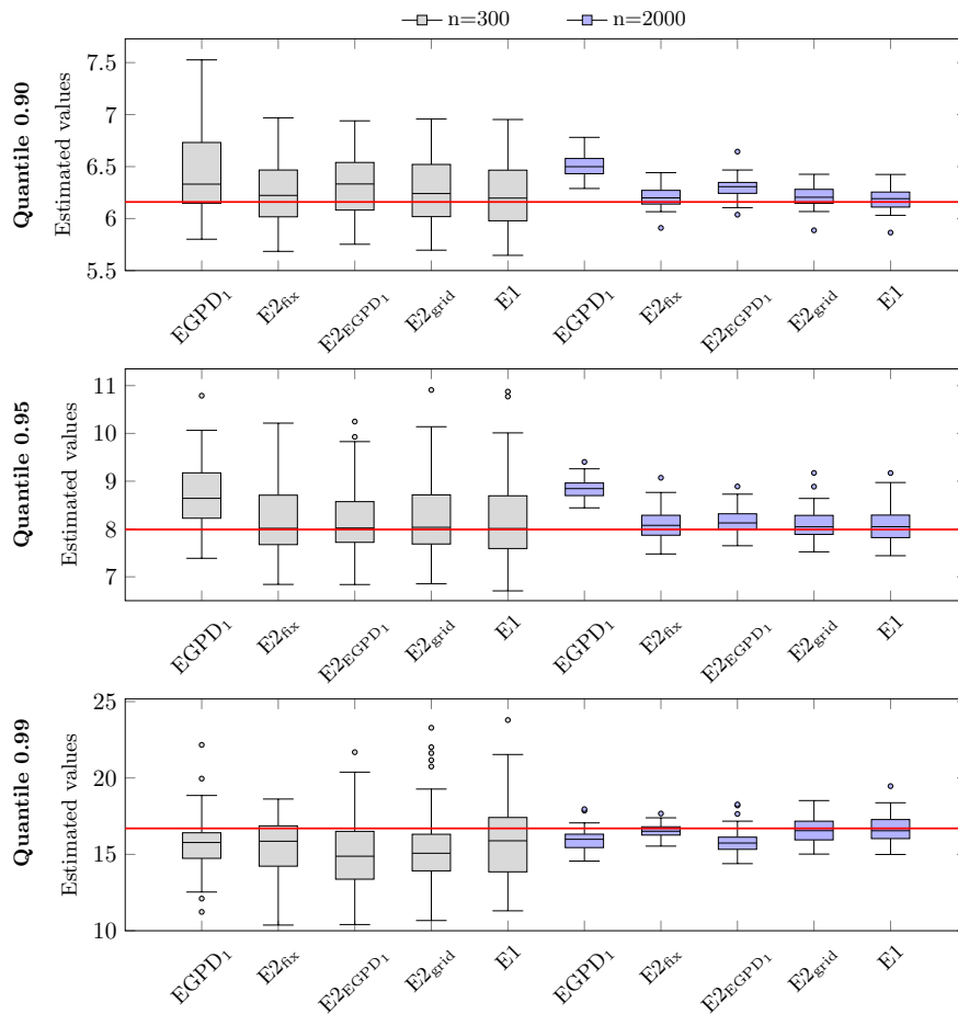
Figure 2.3.5: Boxplots of the estimated q_{0.9} , q_{0.95} , q_{0.99} quantiles of both EGPD 1 and EGPD-BB (with estimation approaches E1, E2 fix , E2 EGPD 1 and E2 grid , and m = m_{\text{true}} ) over 50 replicates, for the sample sizes n = 300 and 2000 (the red horizontal line indicates the true value of the quantiles)
