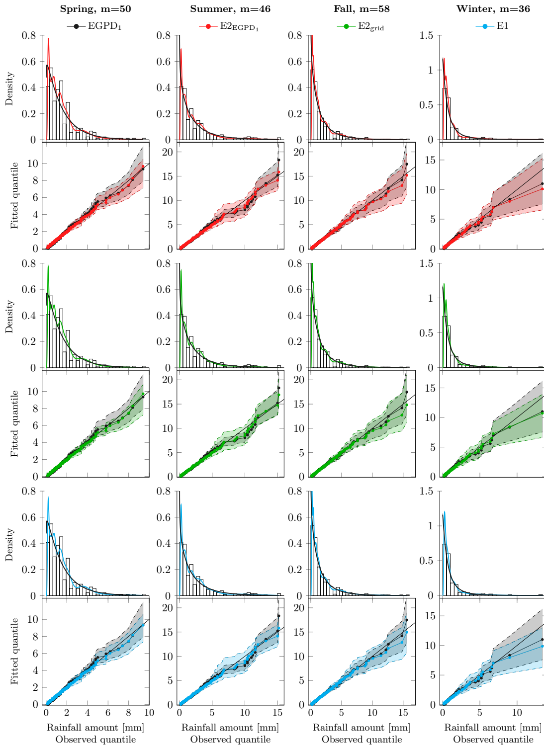
Figure 2.3.9: Histograms with the fitted densities and QQ-plots with the associated 95% confidence intervals for EGPD 1 and EGPD-BB with m = m_{\text{opt}} for hourly Lyon rainfall data (1996–2011), for each of the four seasons. Three approaches are considered for the estimation of the EGPD-BB model: E1, E2 EGPD 1 and E2 grid
