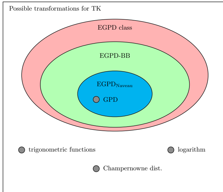
Figure 2.4.1: The general EGPD framework and its relationship with the proposed model: EGPD-BB and TK
