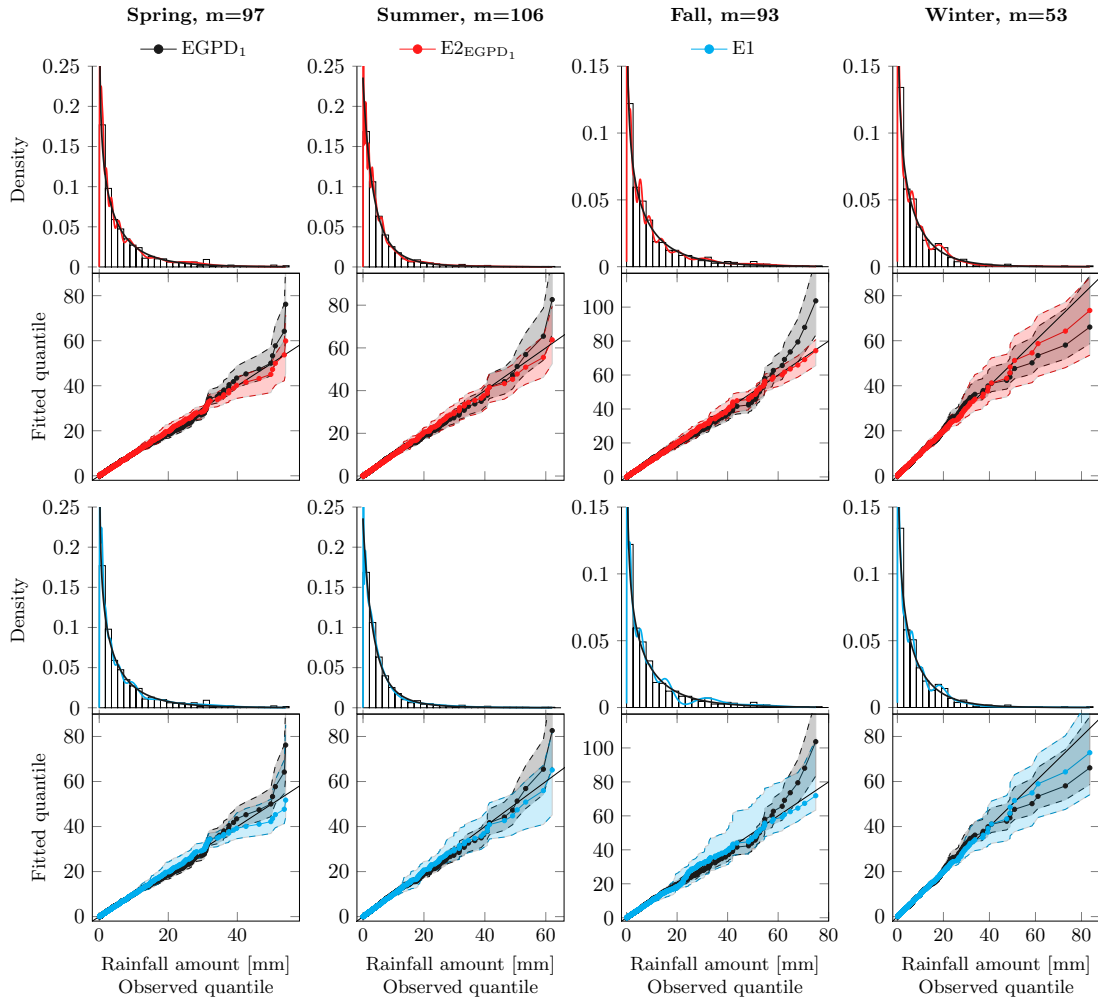
Figure 2.3.15: Histograms with the fitted densities and QQ-plots with the associated 95% confidence intervals for EGPD 1 and EGPD-BB with m = m_{LSCV} for daily Durance rainfall data (1948-2010), for each of the four seasons. Two approaches are considered for the estimation of the EGPD-BB model: E1 and E2 EGPD 1
