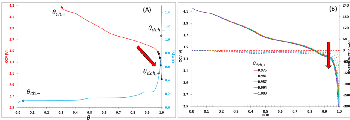
Figure 71 – The isotherms of the LGC INR18650MH1 cell are reported in (A) and the complete cell open circuit voltage and the differences between the initial OCV and OCV with shifted stoichiometry are reported in (B). This scenario illustrates the consequences on the OCV if the \theta_{dch,+} increase because of the cell degradation as indicated by the red arrows.
