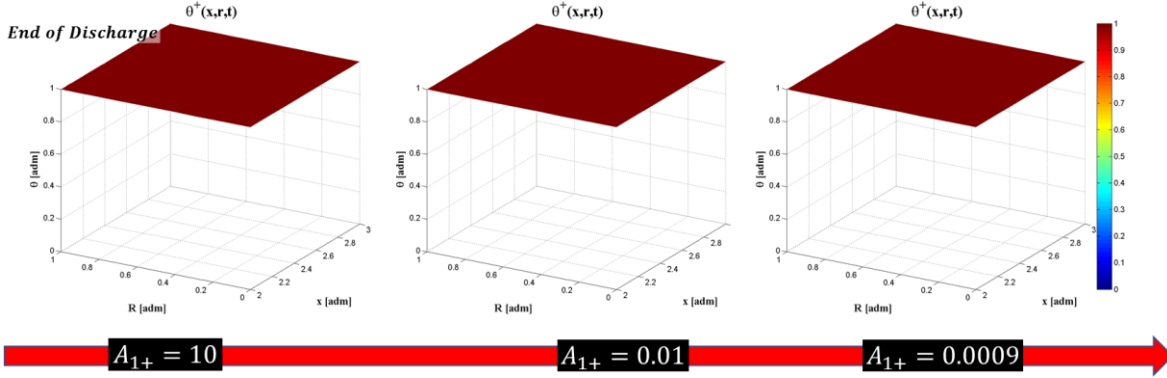
Figure 100 – The profile of the solid phase concentration in the positive electrode (the axis in the bottom of the figures are the electrode thickness and particle radii) is reported at the end of discharge. The red arrow indicate the direction of smaller A_{1+} .
