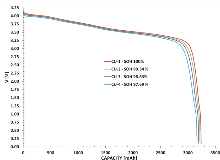
Figure 45 – The discharge voltage is reported as a function of the capacity for the C/3 discharges used to calculate the battery capacity before each test sequences. The state of health is reported and calculated using the first rated capacity at C/3 as reference.
