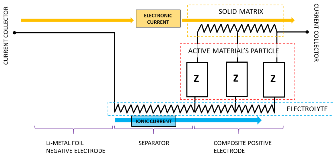
Figure 94 – The general representation of the Transmission Line Model (TLM) for the half-cell is reported. The impedances represents the diffusion in the active material particles, and the resistances the voltage drop in the electrolyte and solid phase matrix. The arrows indicate the ionic current and the electronic current, respectively.
