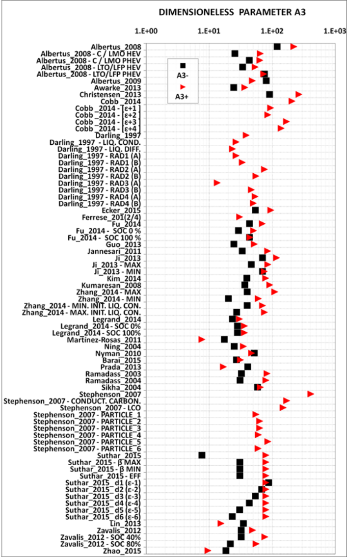
Figure 30 – The dimensionless parameter A_3 is associated to the amount of active material in the electrode.
