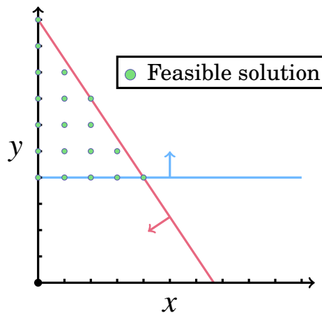
Figure 3.2 – An ILP representation of the problem from Figure 3.1. There are only nineteen valid solutions this time, instead of an infinity.
