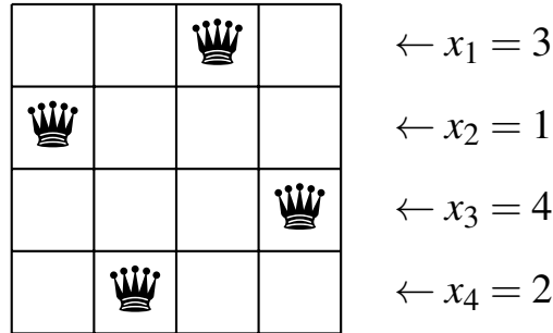
Figure 2.1 – A solution to the 4-queens problem.
