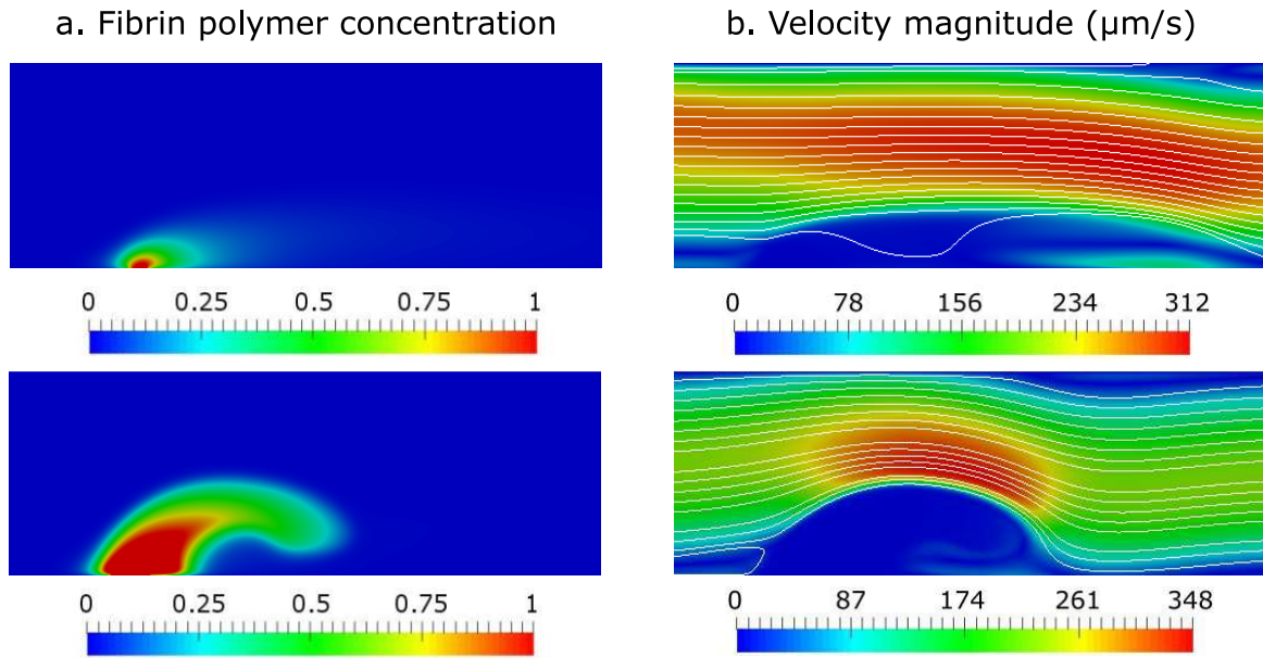
Figure 3.1: Snapshots of simulations for D_a = 2.24 at t = 100 s (top) and t = 640 s (bottom) of thrombus development resulting in complete occlusion. A microvessel of 250 \mu m length is considered where the area of the damaged part is equal to 10 \mu m . Blood flow is not sufficient to stop clot growth (initial velocity is v = 400 \mu m/s ). APC does not allow clot growth width but it still grows across the flow. a) Fibrin polymer concentrations are shown at two consecutive moments of time. b) The corresponding flow velocity fields are shown with the velocity value (color scale) and streamlines (white curves).
