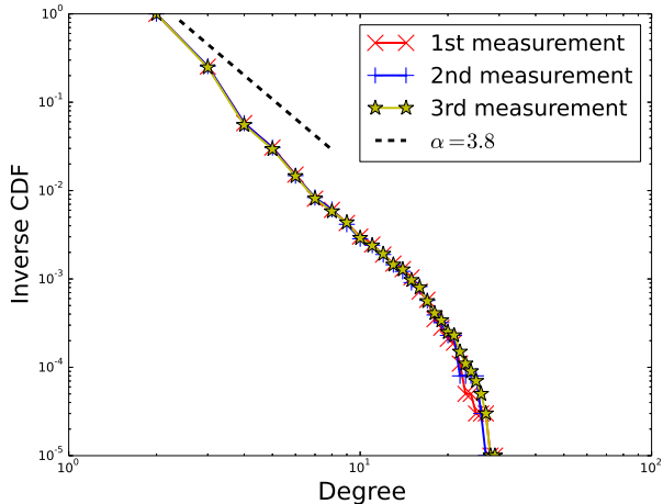
Figure 1.5: Inverse cumulative degree distributions obtained from our three measurements, after bias correction. For each value x on the horizontal axis, we plot the fraction of core routers having degree higher than or equal to x (log-log scale). We also plot the power law of exponent \alpha = 3.8 to show that obtained distributions are incompatible with a power law of exponent lower than this.
