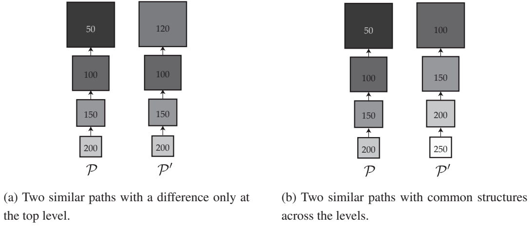
Figure 3.4: Example of similar paths \mathcal{P}, \mathcal{P}' with a certain level transformation.
