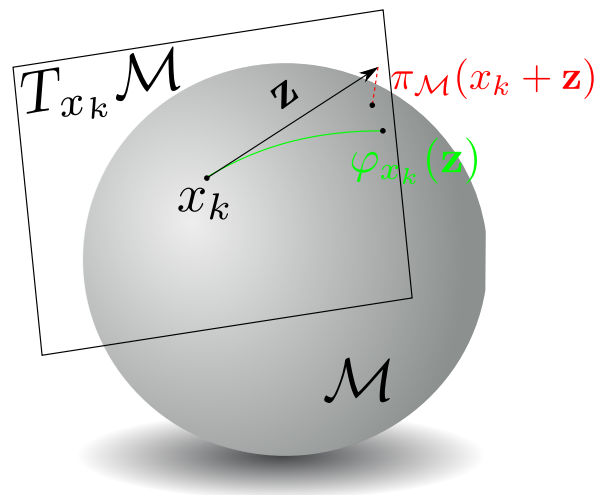
Figure 4.1 StepOnSphere
