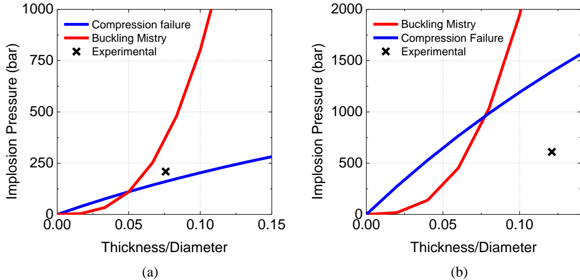
Figure 130 : Implosion pressure versus the thickness to diameter ratio – Simple buckling (Mistry) and strength prediction compared to the experimental implosion pressures for the C/PA6 cylinders laid at (a) [\pm 55] and (b) |0/\pm 88]
