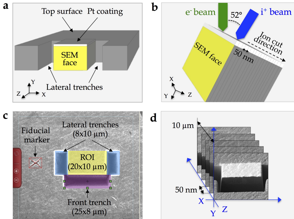
Figure 57: Schematic illustration of the serial sectioning procedure by dual-beam FIB: (a) front view and (b) lateral view of the 52°tilted sample inside the FIB chamber. (c) Slice and View FEI software interface for the preliminary trenching preparation. (d) Stack of SEM images with a z-spacing of 50 nm, through 10 μm (200 images in total).
