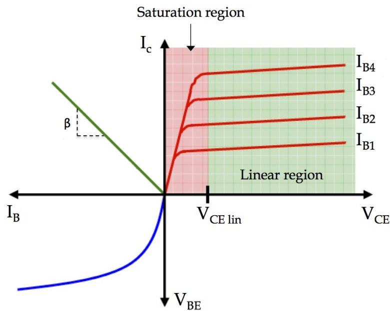
Figure 4: Electrical characteristic curves of a NPN bipolar junction transistor. The blue curve corresponds to V_{BE} = f(I_B) . The red curves correspond to I_C = f(V_{CE}) at increasing I_B values. The red area ( V_{CE} < V_{CE\ lin} ) indicates the saturation region whereas the green one ( V_{CE} > V_{CE\ lin} ) the linear region. The green curve corresponds to I_C = f(I_B) . \beta is the curve slope, that is the device gain.
