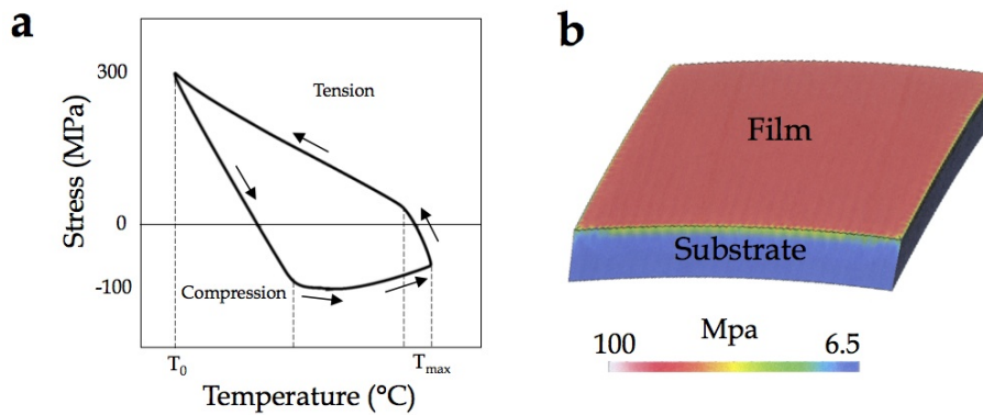
Figure 19: (a) Typical stress-temperature cycle for a 1- \mu m-thick poly-crystalline Al film on oxidized Si substrate ( T_{max} \sim 450^\circ\text{C} ). (b) Finite element simulation showing the Von Mises stresses generated by a temperature change of 50 °C in a 1 cm x 2 cm x 0.5 mm specimen (typical size used in wafer curvature) [Leg09].
