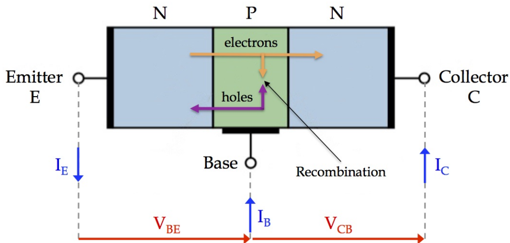
Figure 3: Bipolar transistor general structure.
