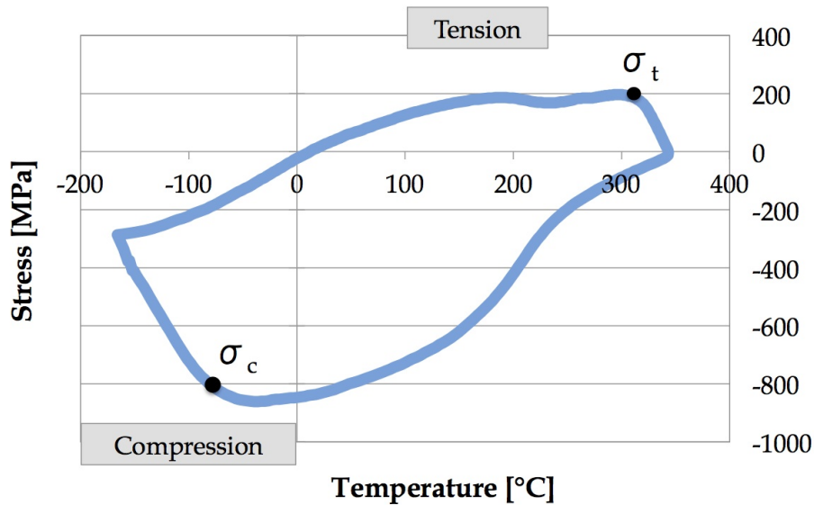
Figure 140: Stress-Temperature cycle for the Al thin film deposited onto the Si wafer. The relative stress is measured along the larger die dimension, and the zero value is here taken at 350\text{ }^{\circ}\text{C} . The cycle is initiated at T = -190\text{ }^{\circ}\text{C} , and the T gradient is set to 20\text{ }^{\circ}\text{C}/\text{min} during heating and cooling.
