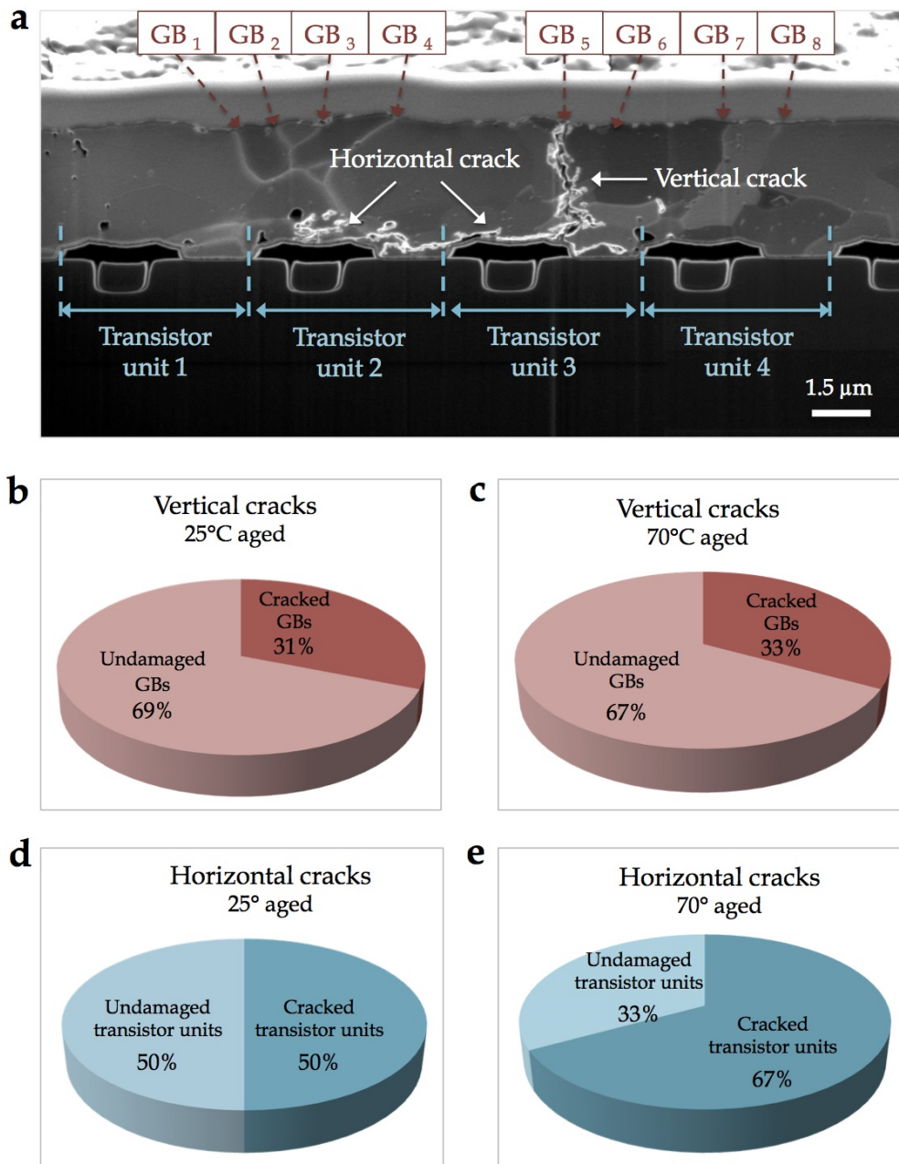
Figure 93: Horizontal and vertical cracks statistics in a 25°C and 70°C aged module.
