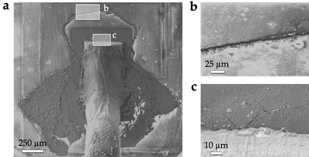
Figure 105: (a) Top view SEM image of an Al bond wire welded on the Al source metallization in a 25^{\circ}\text{C} aged device, after a short-circuit event. At higher magnification, big cracks propagating in (b) the passivated metallization and (c) next to the bonding wire (located in the boxes (b) and (c) in (a)).
