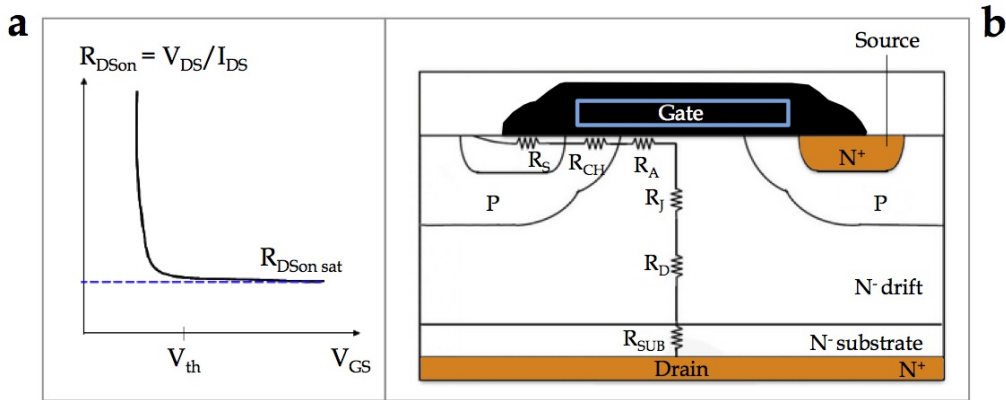
Figure 22: MOSFET vertical structure, showing the total resistances that make up R_{DS(on)} .
