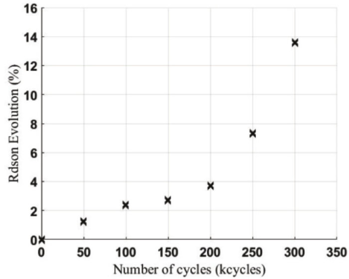
Figure 119: Increase of about 14% in the on-state resistance after repetitive SC events ( 3.55 \text{ J/cm}^2 ) at ambient temperature. At 300kcycles the device failed.
