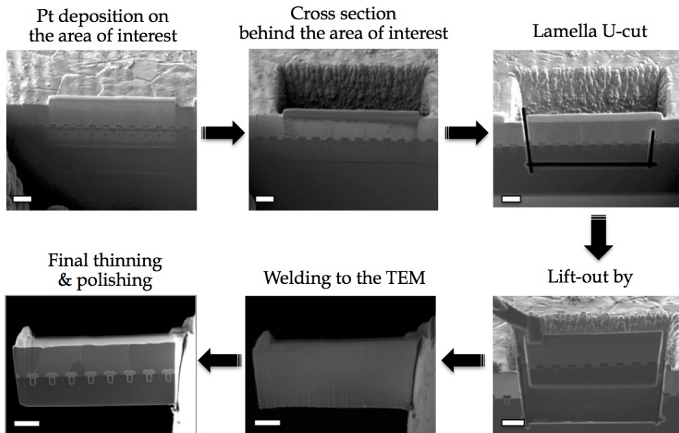
Figure 67: Summary of a FIB lamella preparation for the TEM inspection of the device top Al metallization. Scale bar 2.5 \mu\text{m} .
