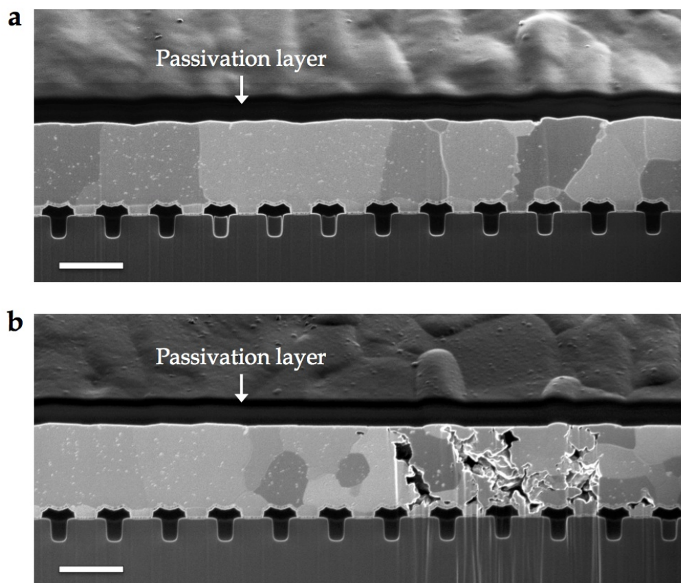
Figure 94: SIM image of the Al top metallization coated by SiO 2 passivation from two close cross-sections in a 70°C aged module.
