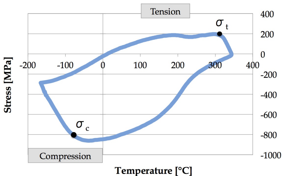
Figure 140: Stress-Temperature cycle for the Al thin film deposited onto the Si wafer. The relative stress is measured along the larger die dimension, and the zero value is here taken at 350\text{ }^{\circ}\text{C} . The cycle is initiated at T = -190\text{ }^{\circ}\text{C} , and the T gradient is set to 20\text{ }^{\circ}\text{C}/\text{min} during heating and cooling.
