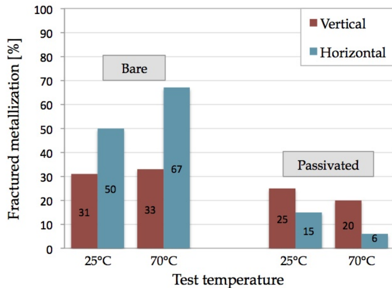
Figure 129: Metallization crack statistics for a To7D17 module aged at 25\text{ }^{\circ}\text{C} and 70\text{ }^{\circ}\text{C} , in non passivated –bare– (left) and passivated (right) zones.
