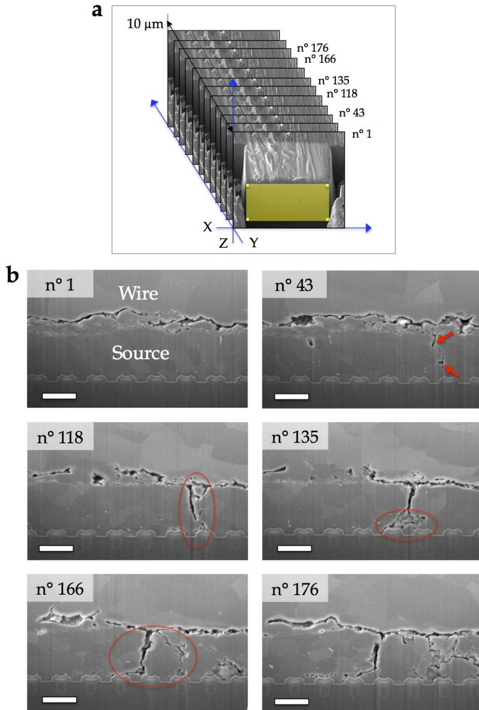
Figure 100: (b) Selection of six non consecutive SEM images from the data stack of the wire-metalization interface (according to the schema in (a)) of a 70 °C aged device (slicing distance 50 nm). The yellow rectangle in (a) represents the milled imaging face. Scale bar 2.5 \mu\text{m} .
