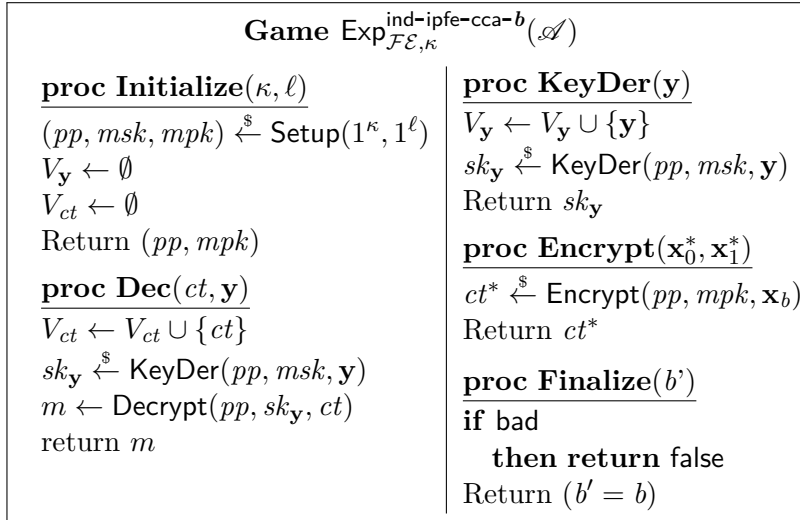
Figure 3.7: Game \text{Exp}_{\mathcal{F}\mathcal{E}, \kappa}^{\text{ind-ipfe-cca-}b}(\mathcal{A}) defines IND-IPFE-CCA security of \mathcal{F}\mathcal{E} . The event bad corresponds to \exists y \in V_y, \langle x_0^*, y \rangle \neq \langle x_1^*, y \rangle \vee ct^* \in V_{ct} .
