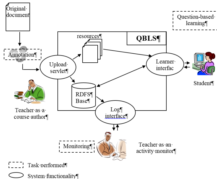
Figure 1.1: Overall QBL approach for creating and exploiting learning resources from available course material
