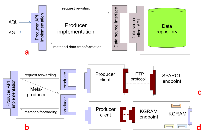
Figure 3.5: KGRAM Producers . Top: regular data source producer. Bottom left: meta-producer. Bottom right: producer towards remote data sources.
