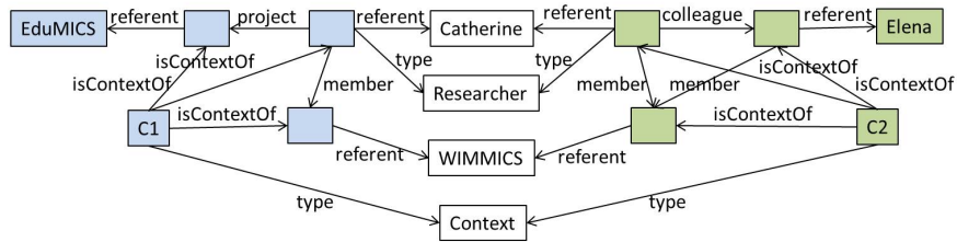
Figure 3.1: Example of an RDF graph embedding two contexts coloured in blue and green; the shared nodes are colourless
