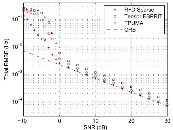
Fig. 7. Frequency total root-mean square error for a 3-D signal containing 3 modes with identical modes in two dimensions (Signal #3), with close modes in the first dimension (0.28,0.12,0.2). (M_1, M_2, M_3) = (10, 10, 10) . 200 Monte-Carlo.
