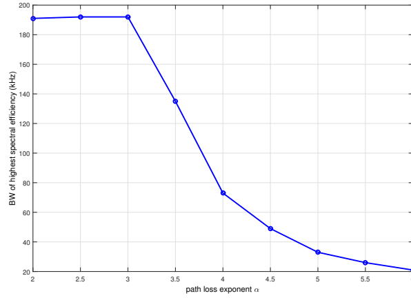
FIGURE 3.34: Bandwidth for highest spectral efficiency ( \frac{N_{max}}{B} ) vs exponent path-loss \alpha , for r_M = 10 km, r_x = 2 km, r_m = 1 m, \gamma^* = 6.8 dB, with guard band
