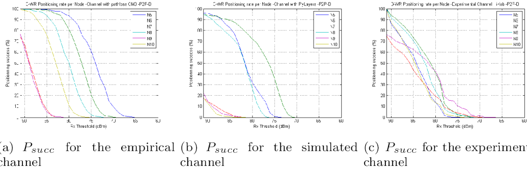
FIGURE 2.26: Success positioning probability ( P_{succ} ) with 3WR and P2P-B.
