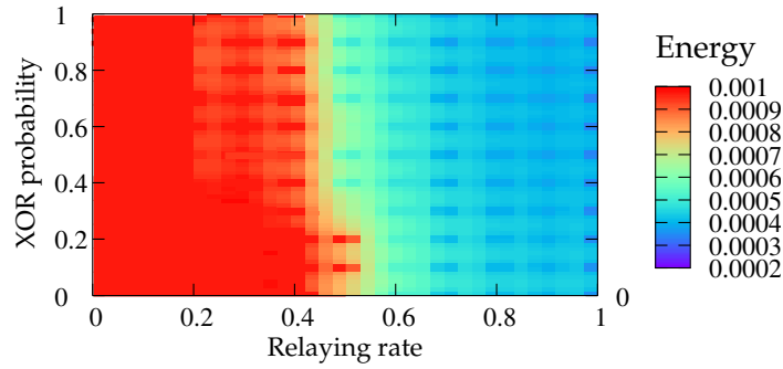
(a) Energy consumption as a function of the relaying rate and the network coding probability
