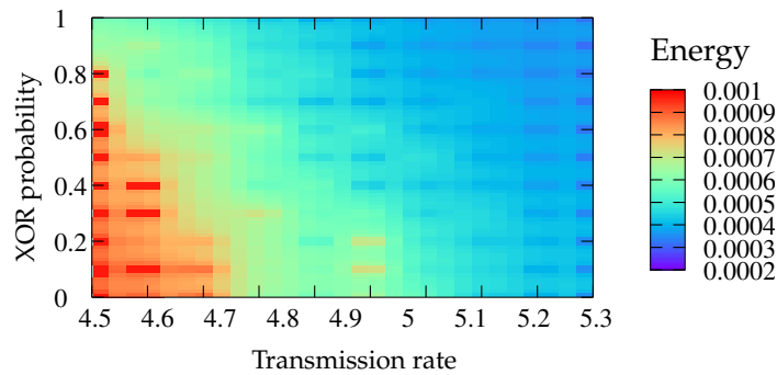
(b) Energy consumption as a function of the relaying rate and the network coding probability for the transition area
