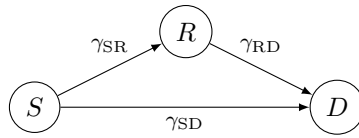
FIGURE 3.13: Relay channel
