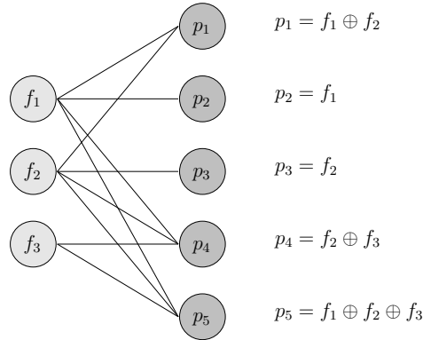
FIGURE 3.2: LT code represented as a bipartite graph
