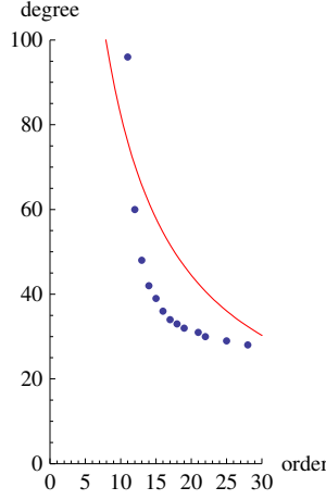
FIGURE 14. Guessing differential operators for G(t; a, 0) , for prime p and a \in \mathbb{F}_p : minimal-order operator (blue point above the hyperbola) obtained as gcd of several non-minimal operators (blue points below the hyperbola). Points below the hyperbola correspond to operators obtainable by Hermite-Padé approximation with 1000 terms.
