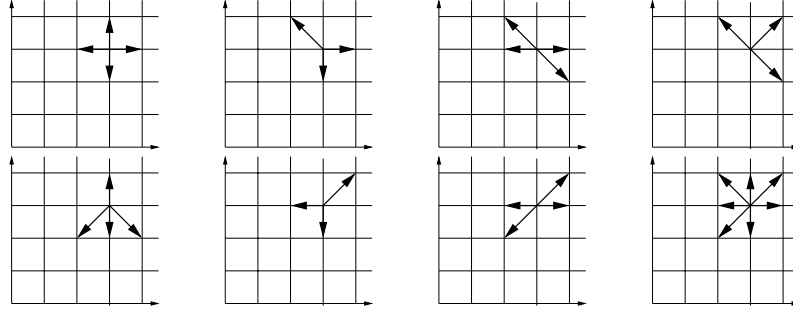
FIGURE 9. Examples of models with groups of orders 4, 6, 8 and \infty , respectively.
